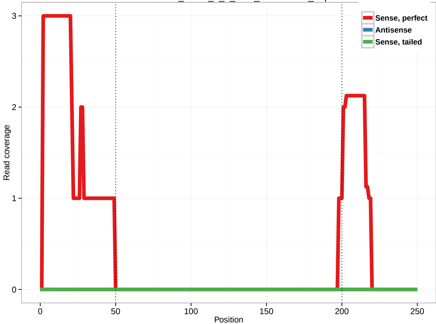
uc001hau.2_intron_8_0_chr1_204214132_r.5p
