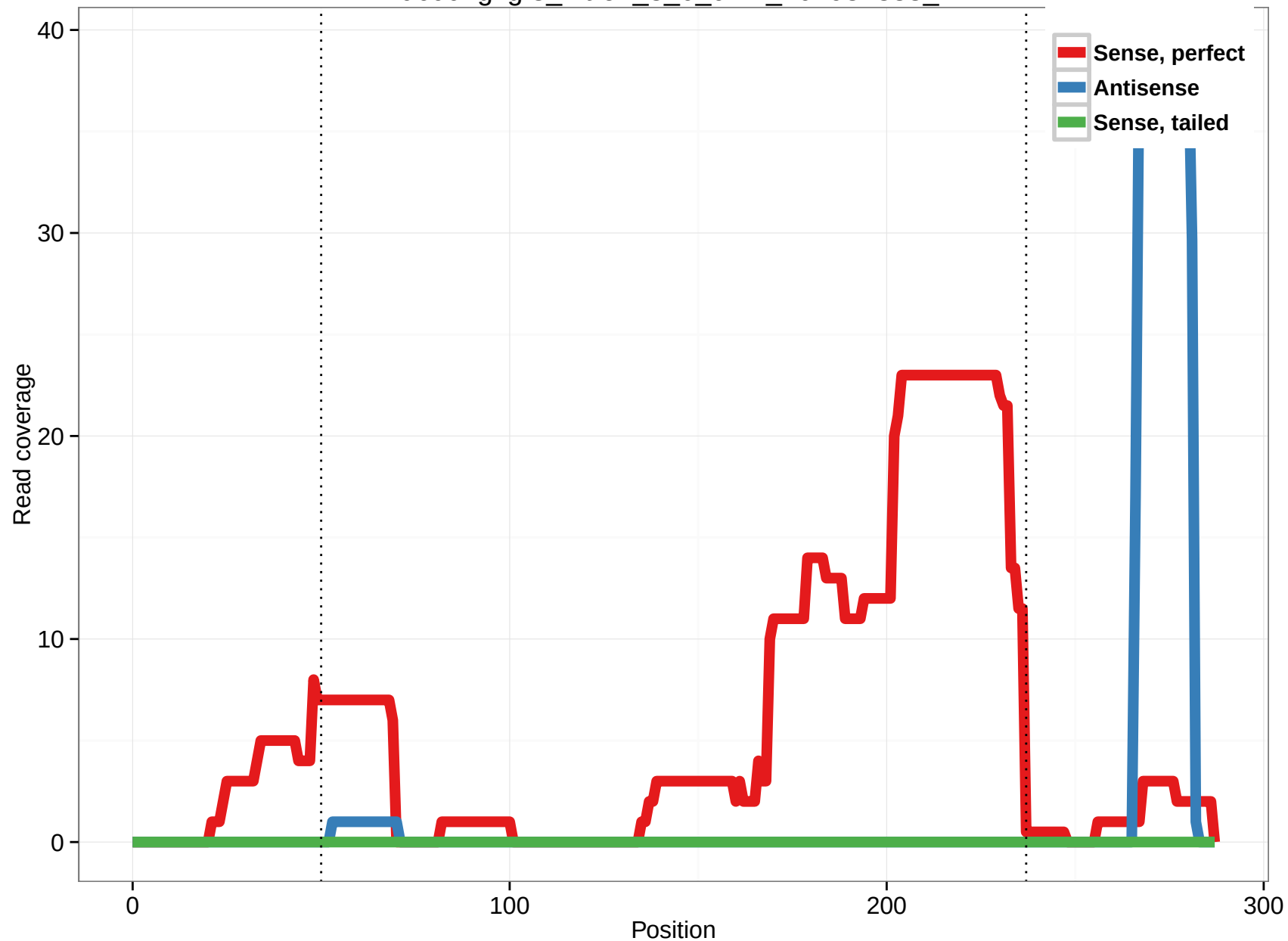
uc001gxcg.3_intron_3_0_chr1_201981888_f
