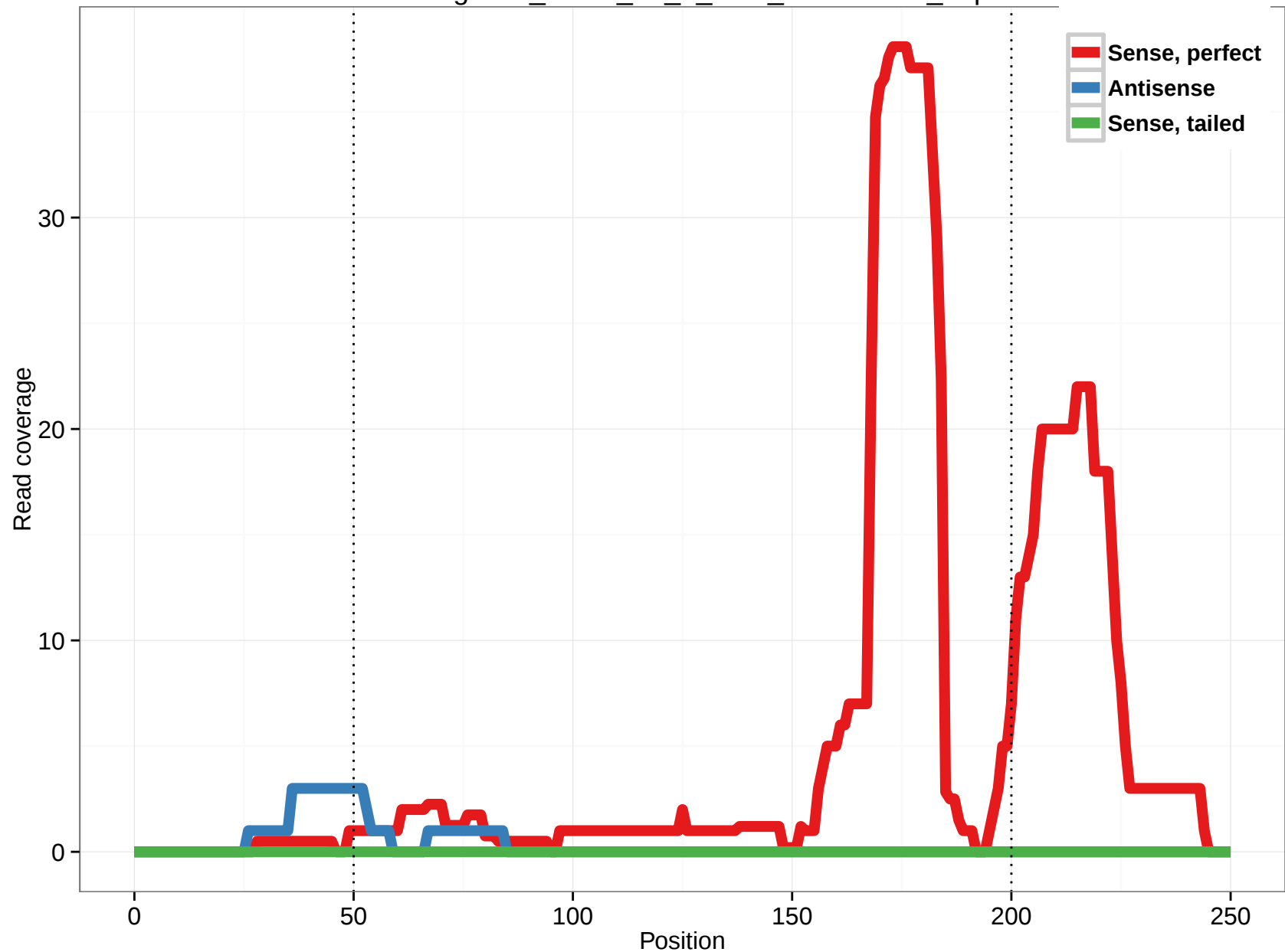
uc001gwd.2_intron_13_0_chr1_201297997_f.3p
