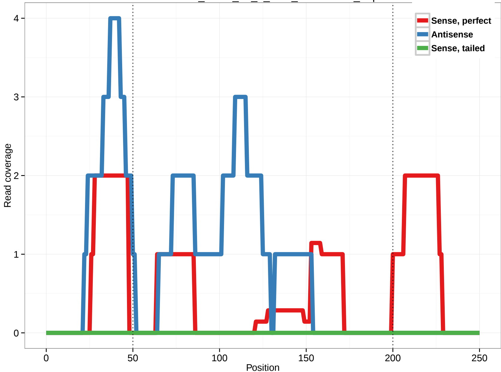
uc001fxf.3_intron_10_0_chr1_160991278_r.5p
