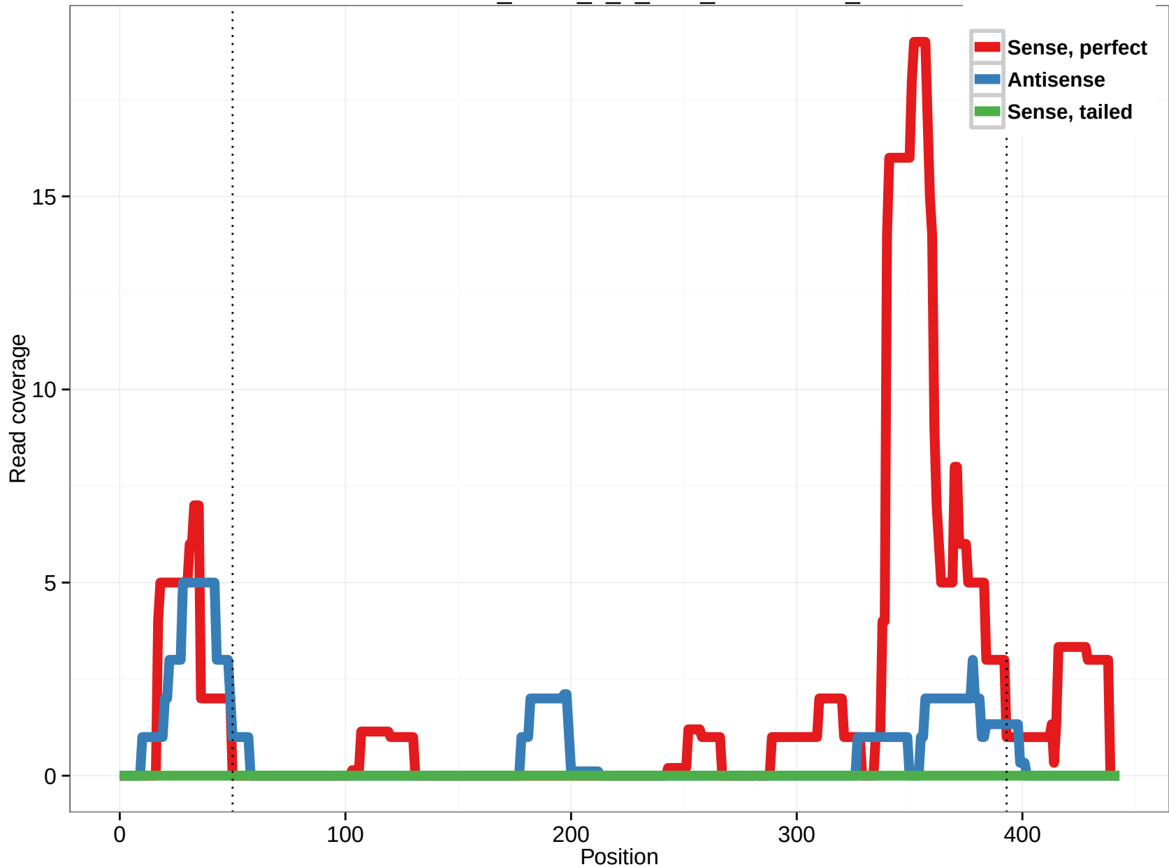
uc001fva.2_intron_1_0_chr1_160061729_r
