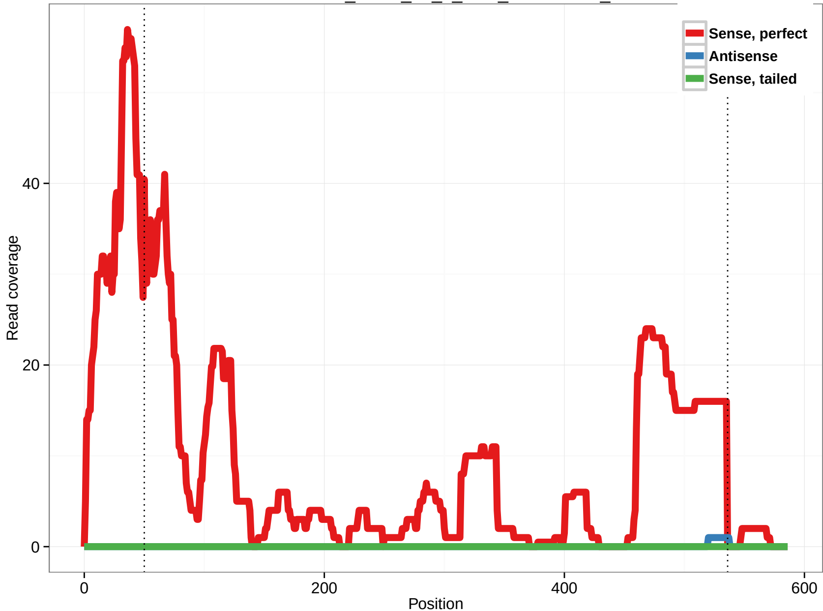
uc001fmi.1_intron_12_0_chr1_155903641_r
