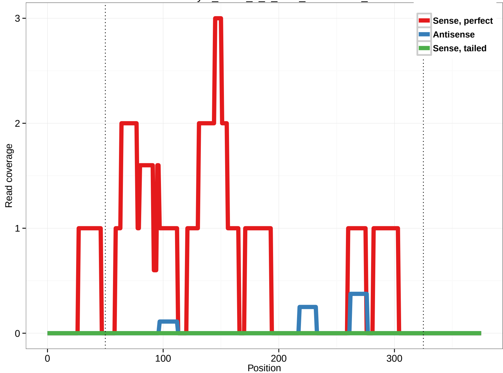
uc001fey.1_intron_5_0_chr1_154304155_f
