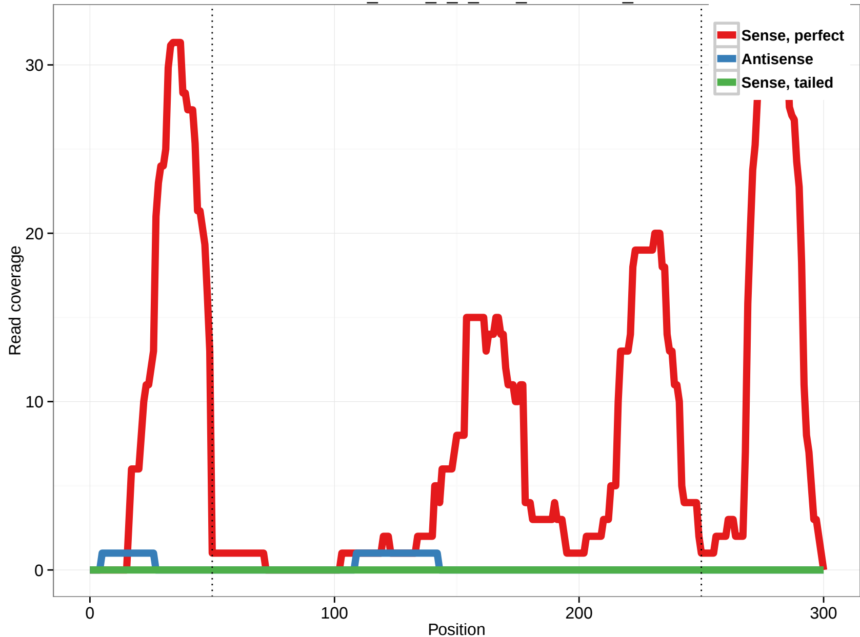
uc001fds.2_intron_2_0_chr1_153949252_r
