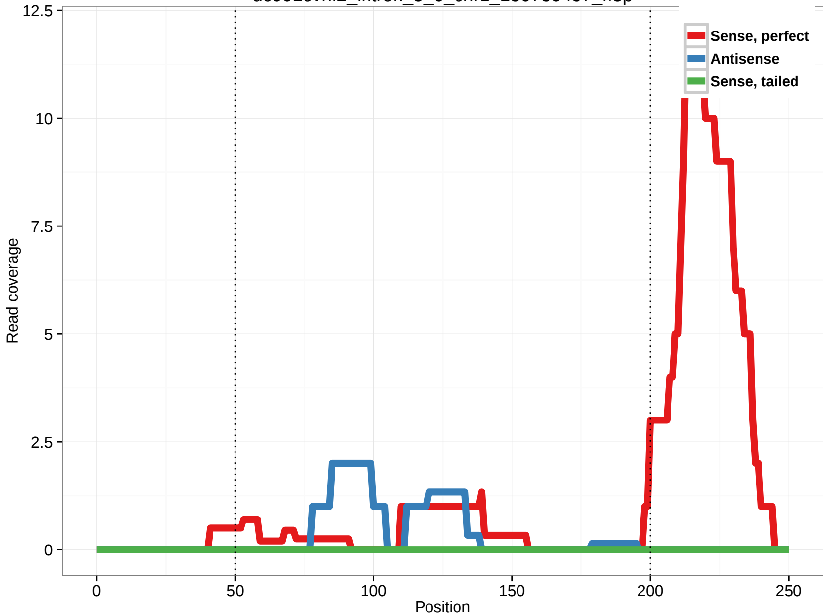
uc001evn.2_intron_5_0_chr1_150730457_r.3p
