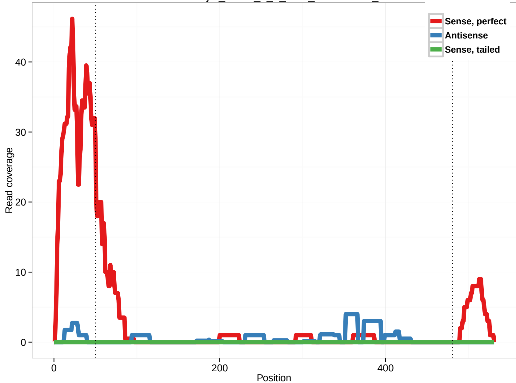
uc001etj.1_intron_4_0_chr1_149899187_r
