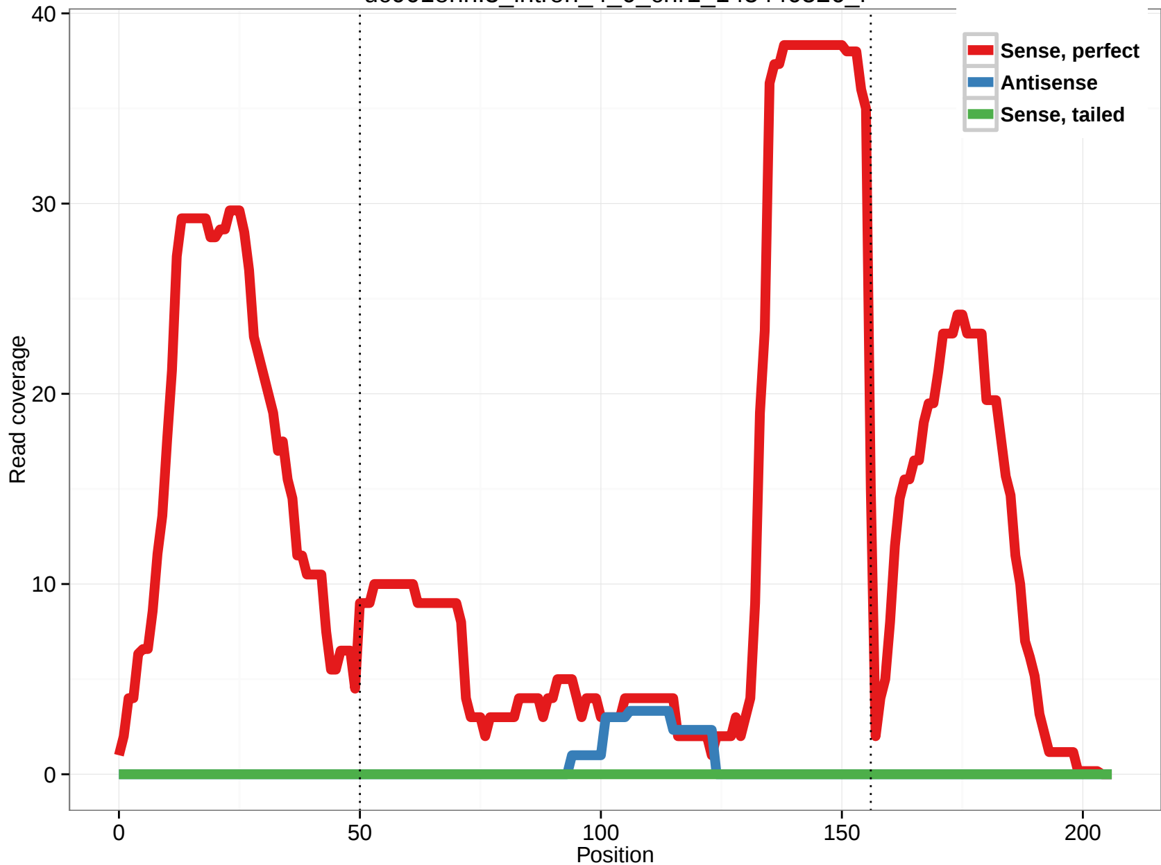
uc001enn.3_intron_4_0_chr1_145440526_f
