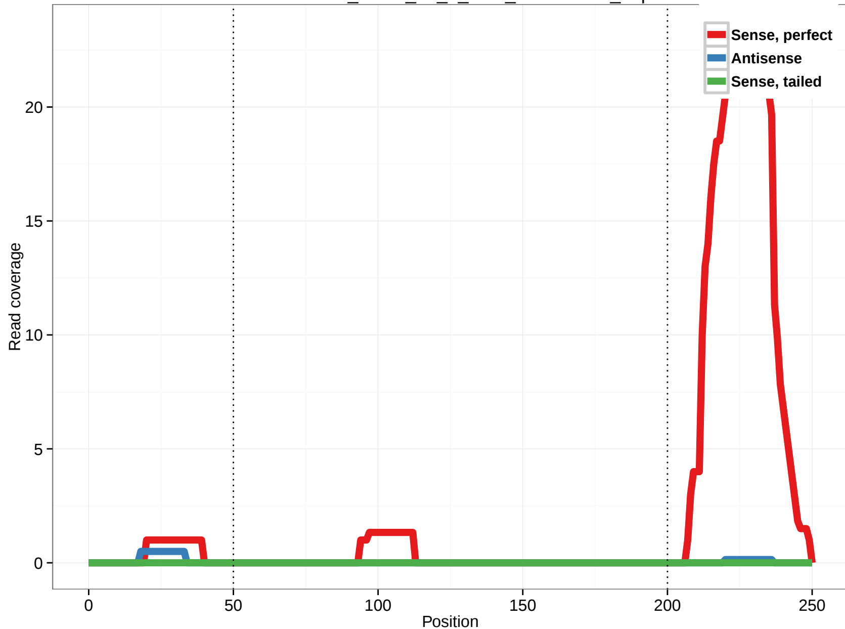
uc001end.3_intron_33_0_chr1_145327666_f.3p
