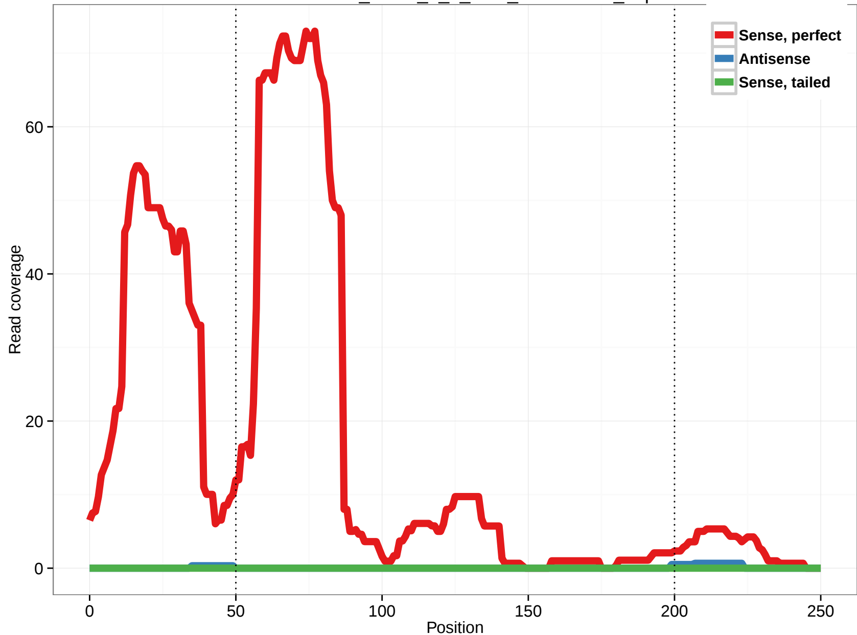
uc001emo.2_intron_3_0_chr1_145281705_f.3p
