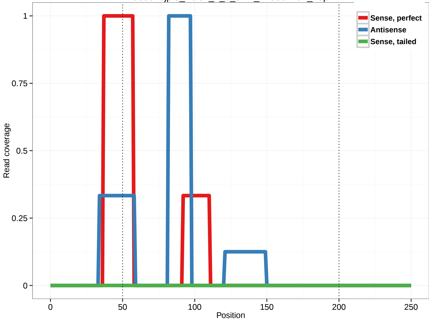
uc001ejp.3_intron_2_0_chr1_143664197_r.3p
