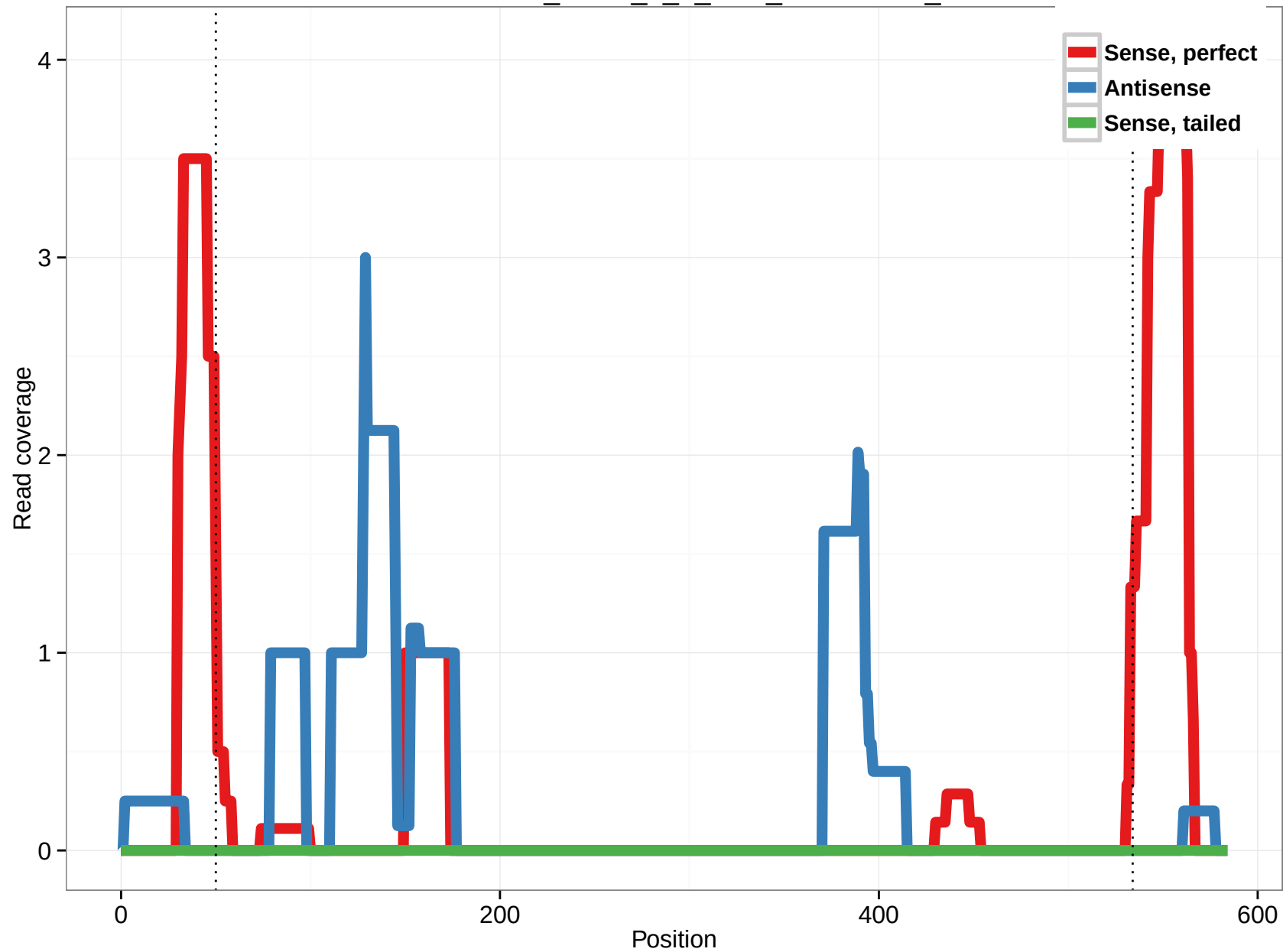
uc001eiw.1_intron_6_0_chr1_143254005_f
