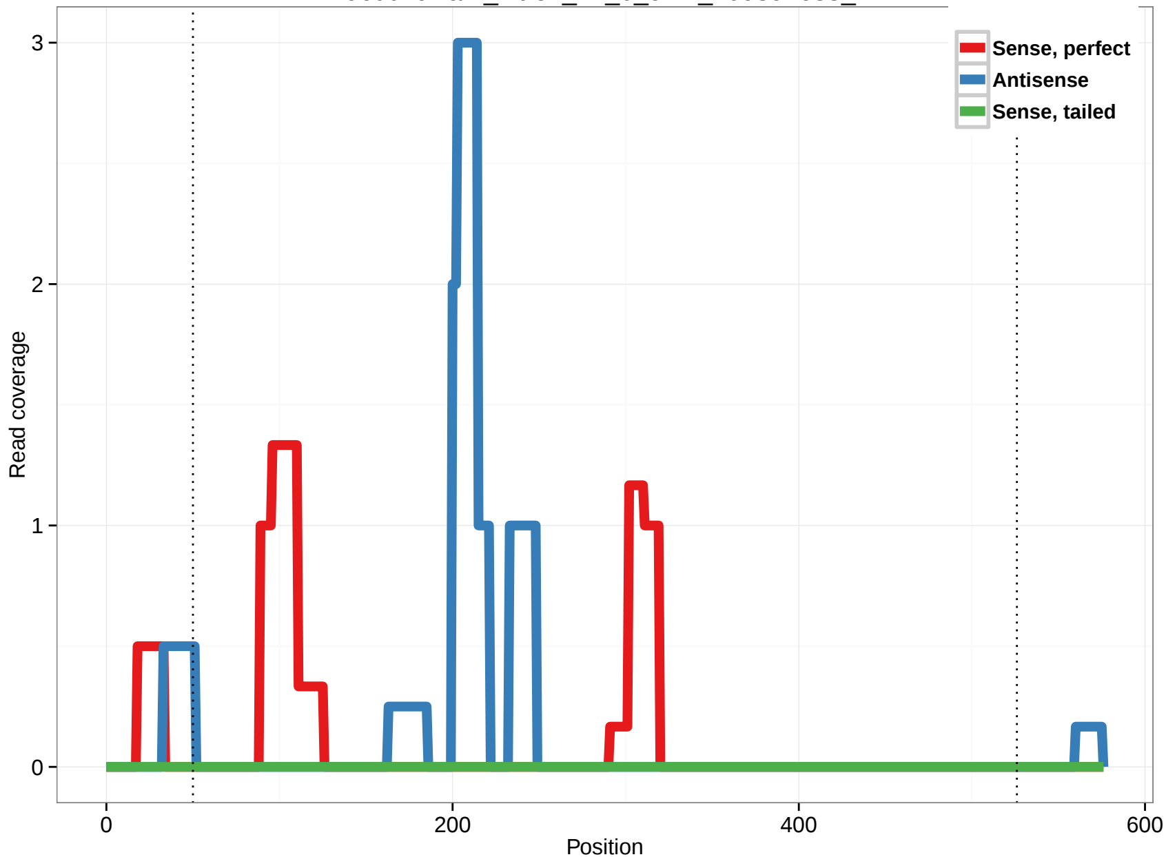
uc001dwa.2_intron_12_0_chr1_109391683_r
