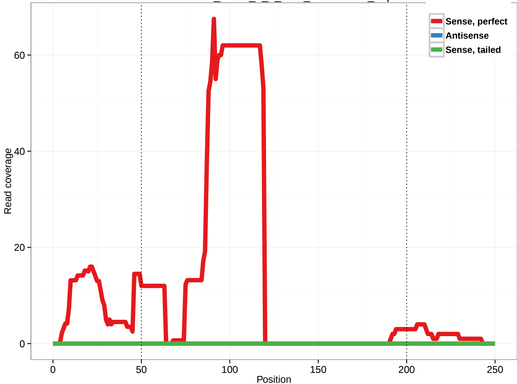
uc001dvv.3_intron_3_0_chr1_109238960_f.5p
