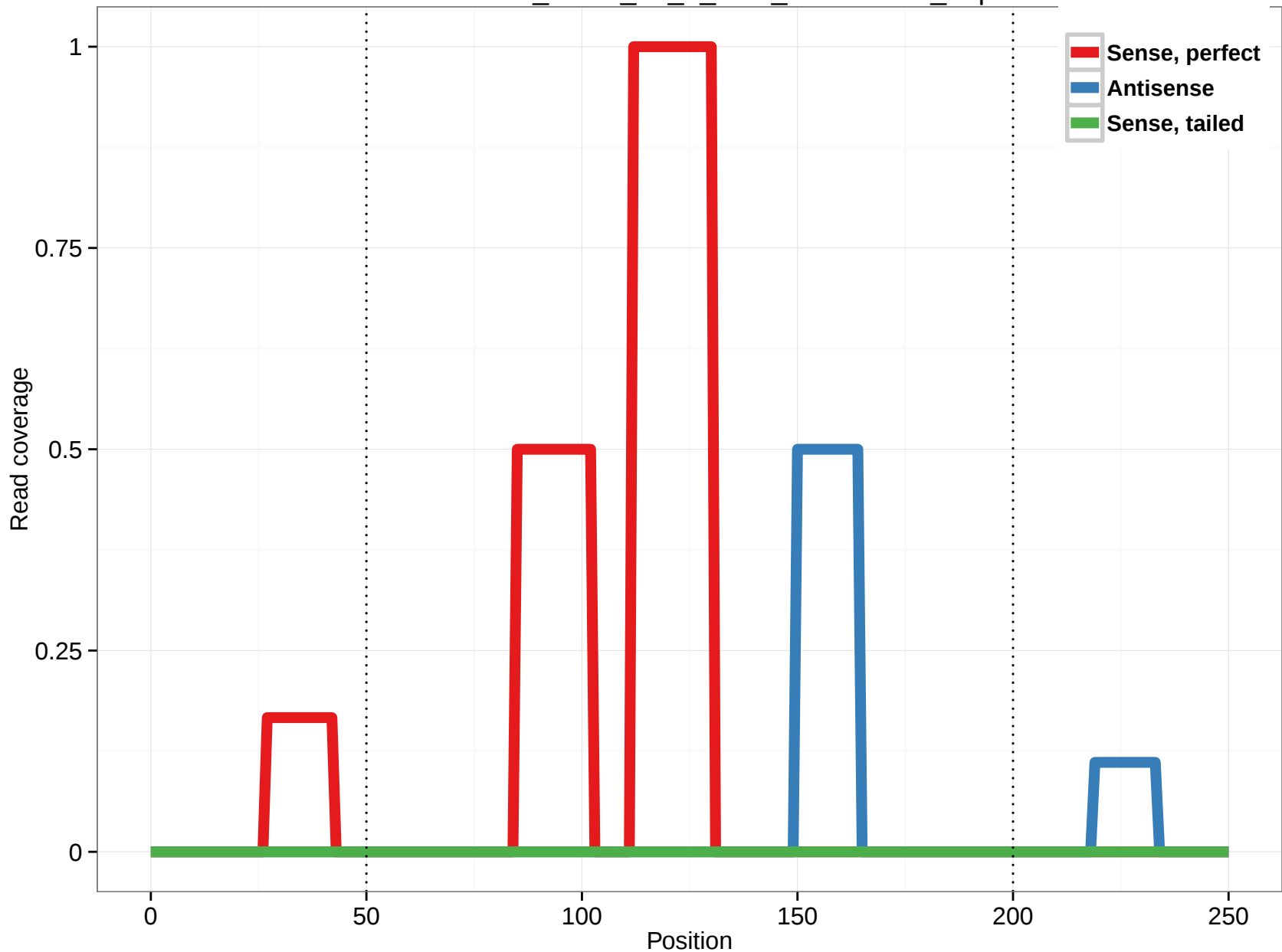
uc001duk.2_intron_39_0_chr1_103455128_r.3p
