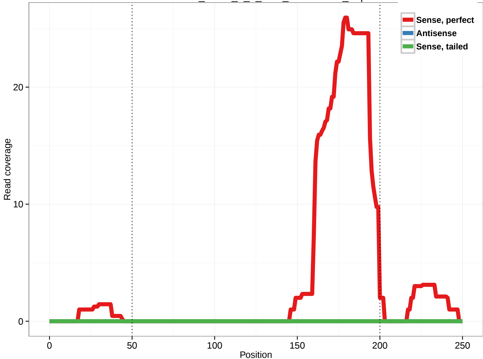
uc001dta.2_intron_0_0_chr1_100661979_r.3p
