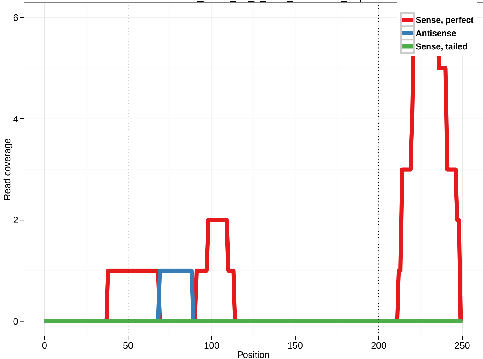
uc001dhv.2_intron_14_0_chr1_78200102_r.3p
