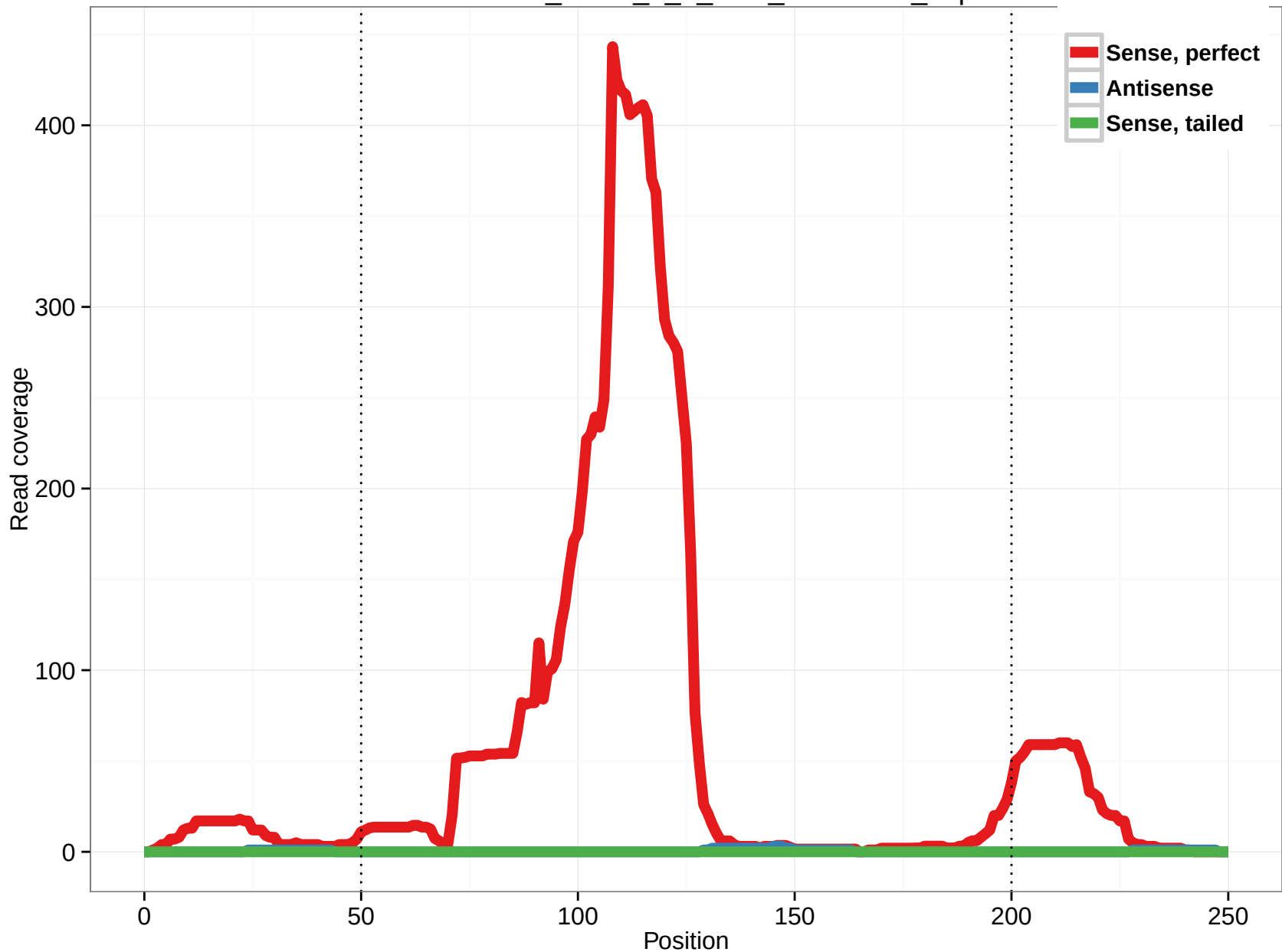
uc001des.2_intron_0_0_chr1_70671464_f.3p
