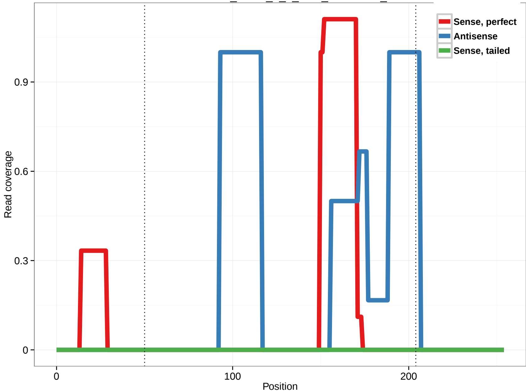
uc001dbk.2_intron_3_0_chr1_64576641_r
