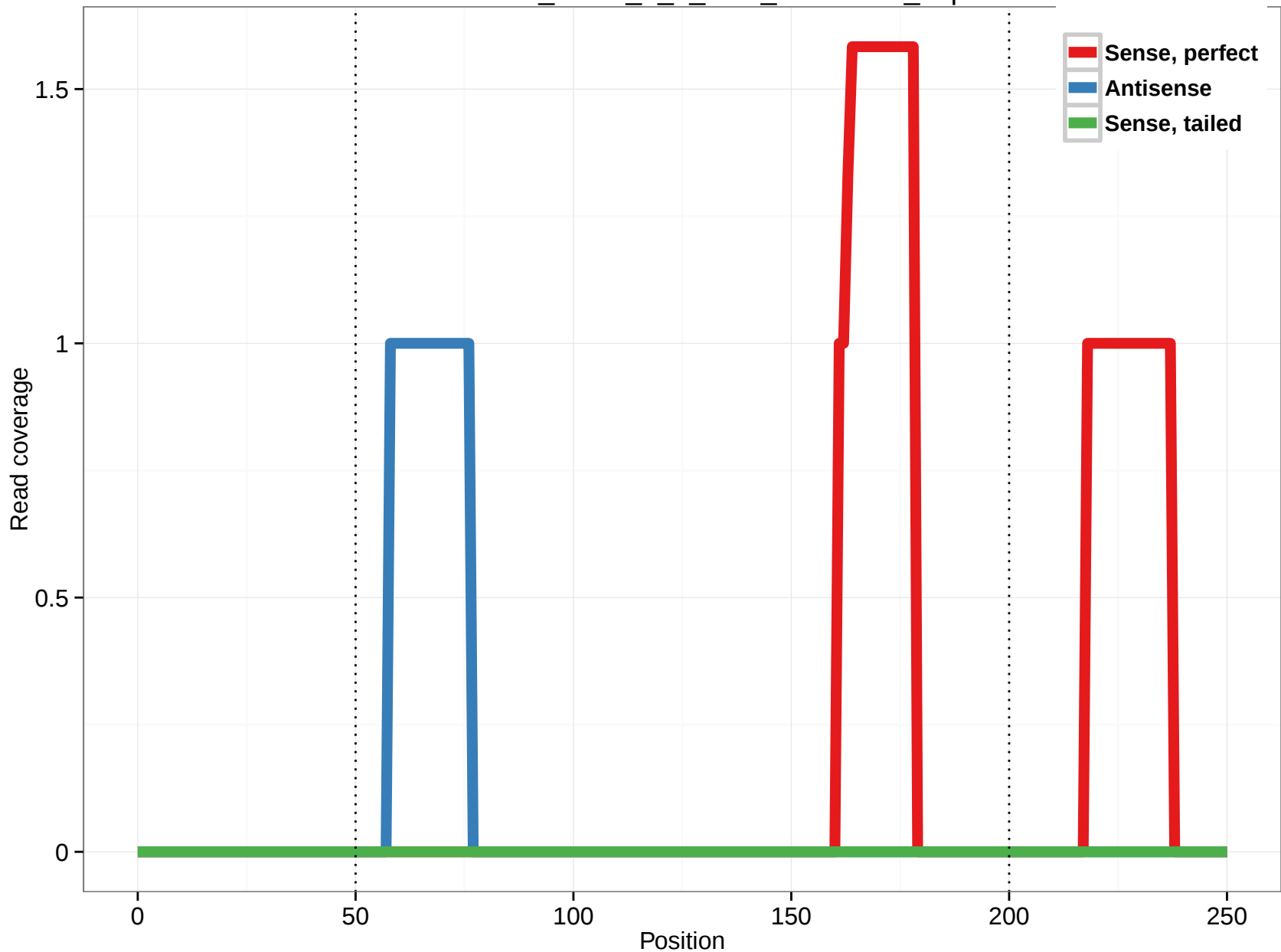
uc001dbf.2_intron_8_0_chr1_64021187_f.3p
