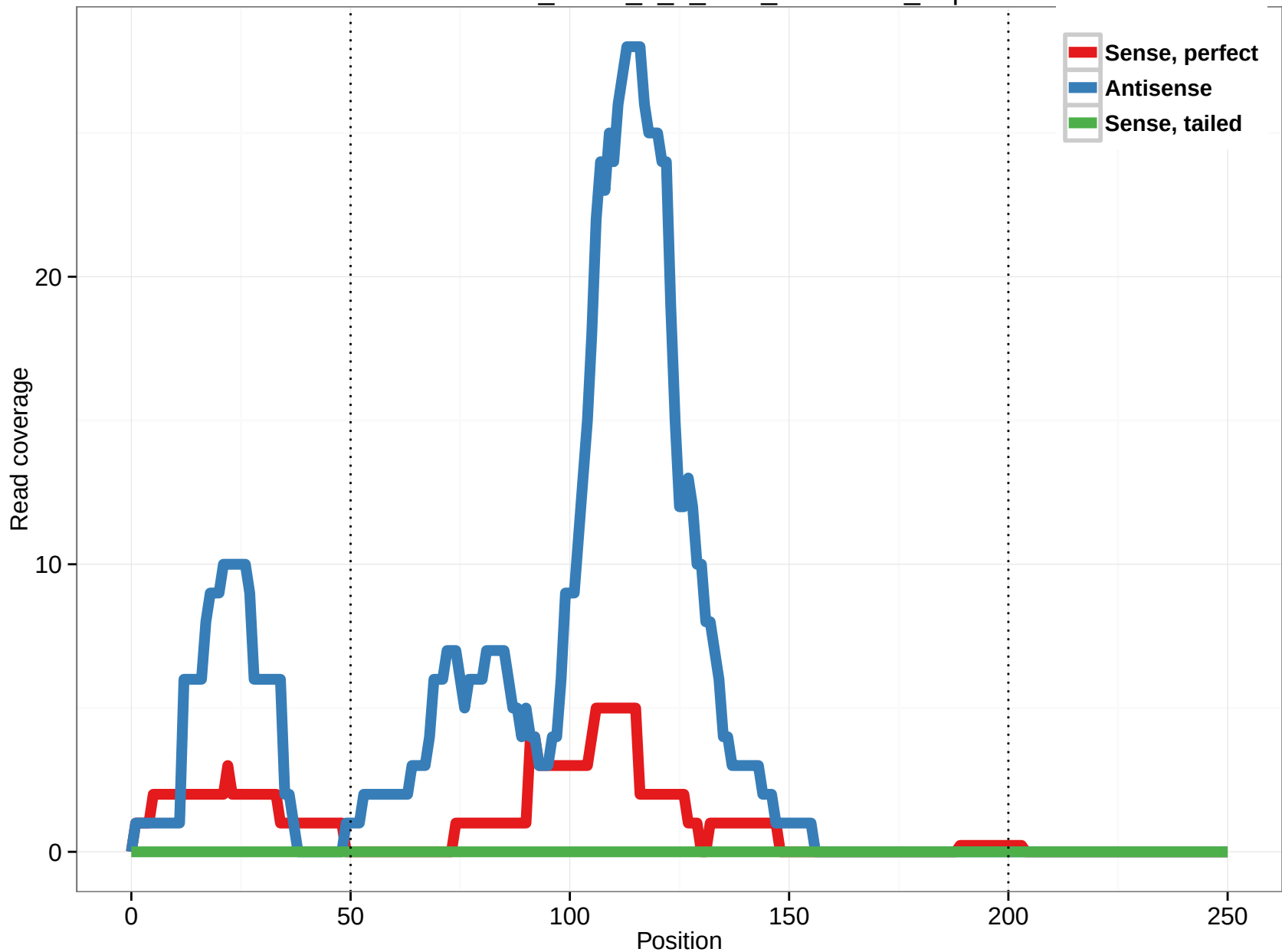
uc001dbc.1_intron_2_0_chr1_63913286_r.3p
