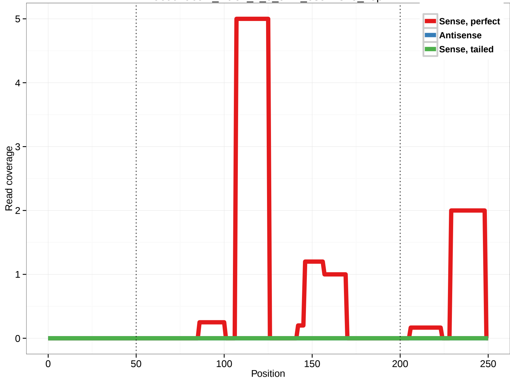
uc001dbc.1_intron_1_0_chr1_63912528_r.5p
