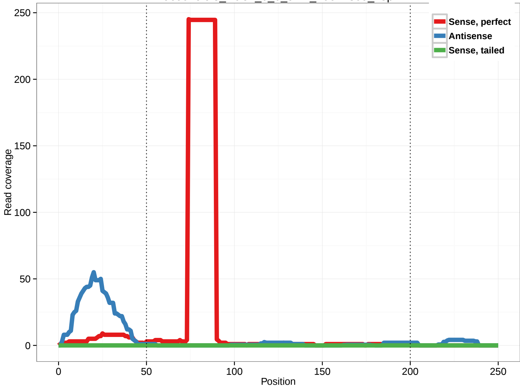
uc001cfc.3_intron_0_0_chr1_40627309_f.5p
