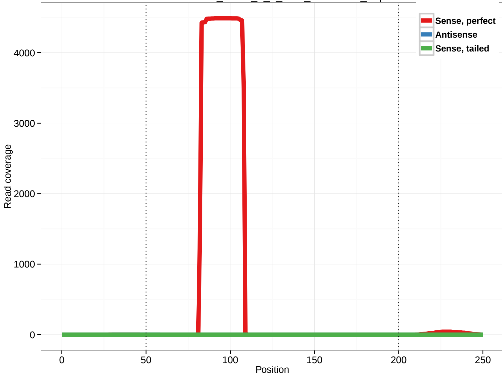
uc001bsc.2_intron_3_0_chr1_31211910_r.3p
