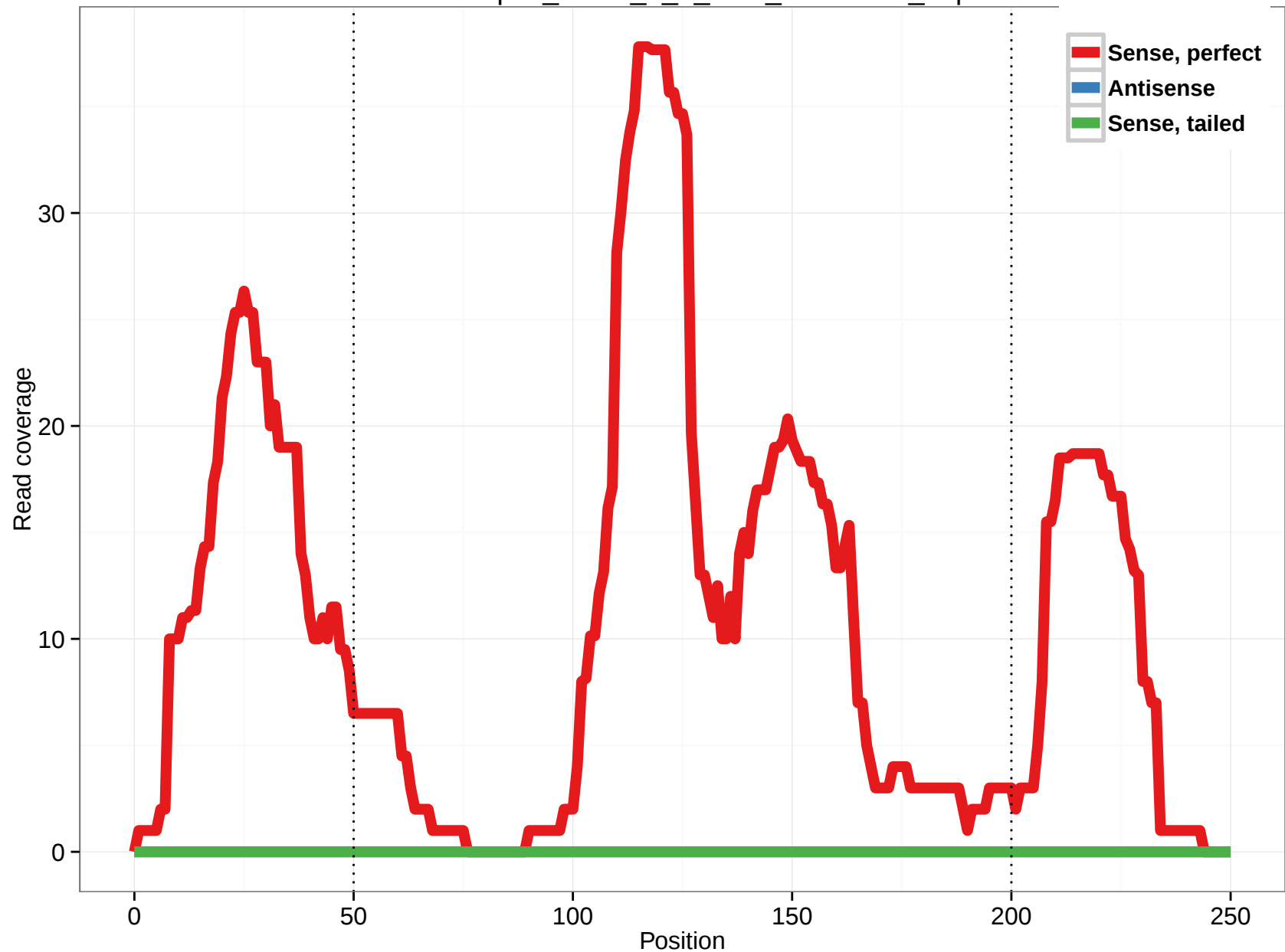
uc001bqa.1_intron_1_0_chr1_28834673_f.5p
