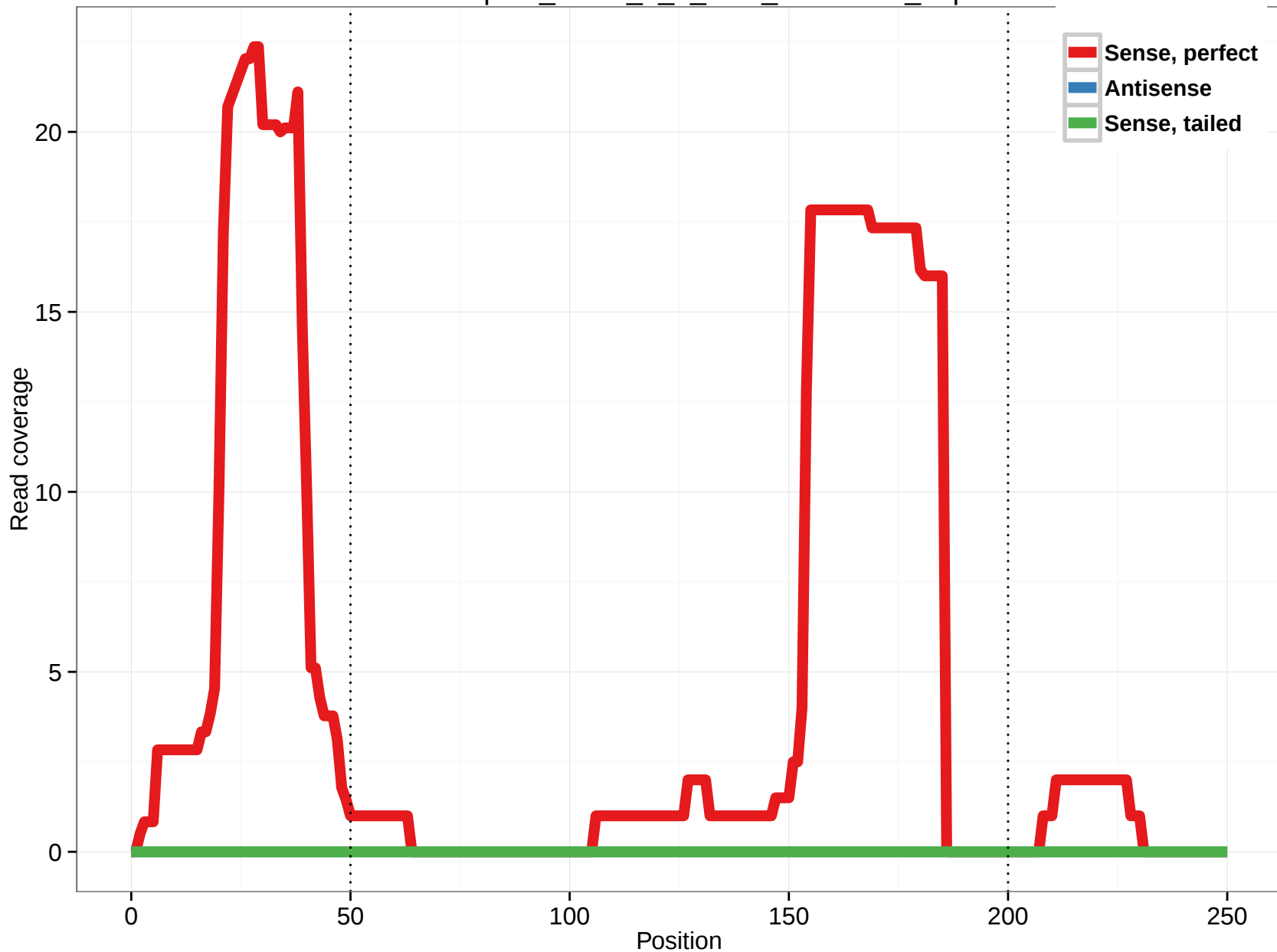
uc001bpn.2_intron_2_0_chr1_28531861_r.5p
