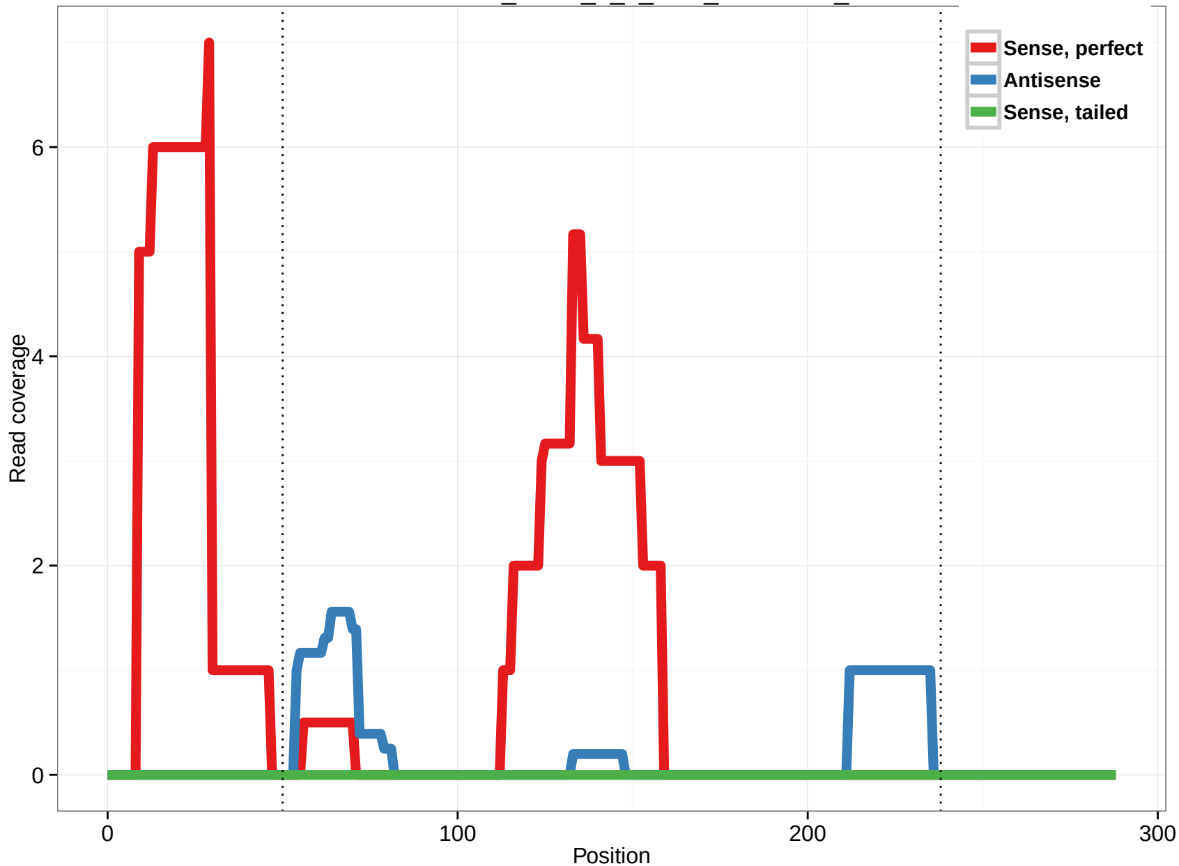
uc001boh.1_intron_0_0_chr1_27878362_r
