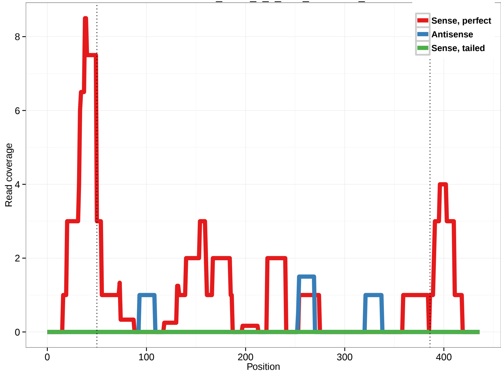
uc001bnz.1_intron_5_0_chr1_27686860_r
