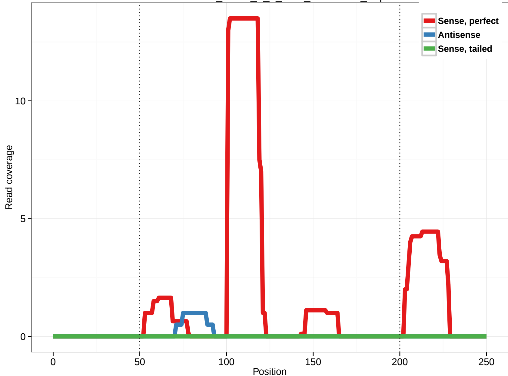
uc001bnm.2_intron_7_0_chr1_27432579_r.5p
