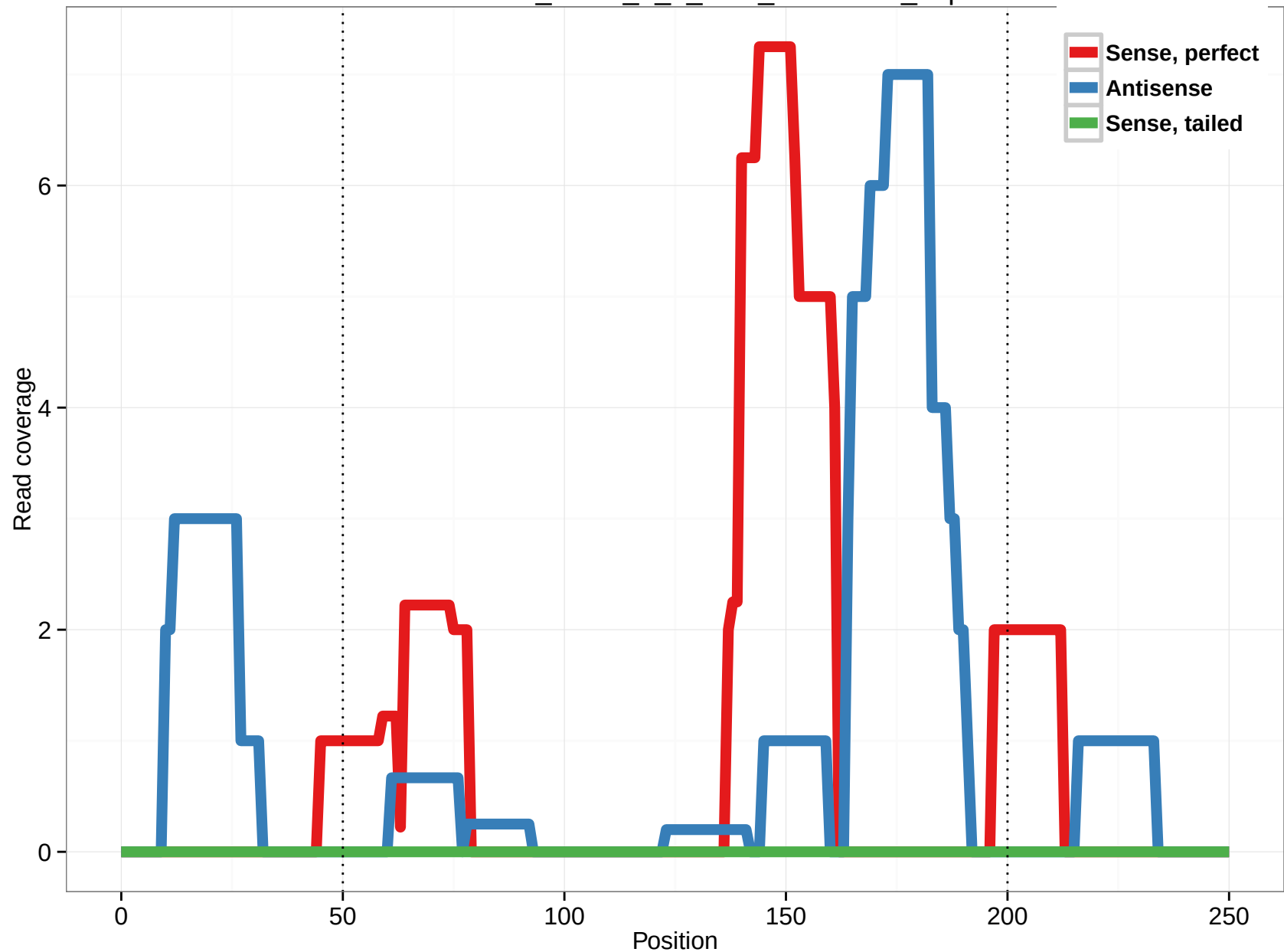
uc001bmr.1_intron_0_0_chr1_26856475_f.5p
