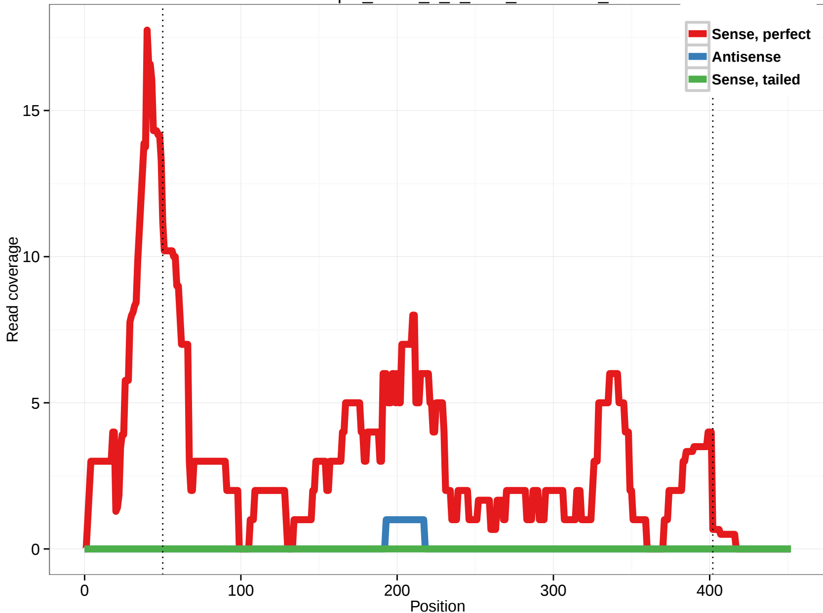
uc001bmp.3_intron_2_0_chr1_26800224_f
