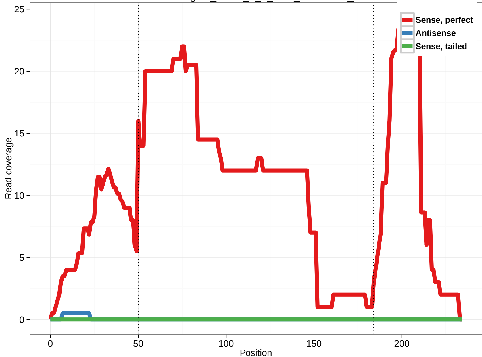
uc001bgo.2_intron_0_0_chr1_23637560_r
