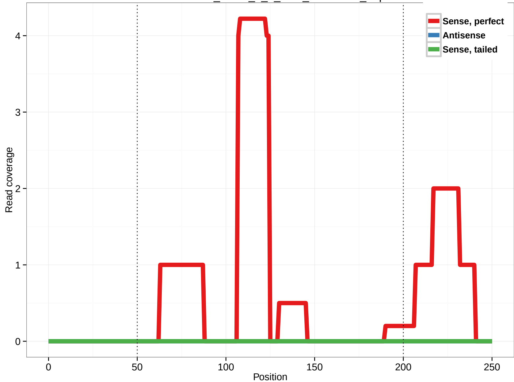
uc001bcz.2_intron_1_0_chr1_20442107_r.3p
