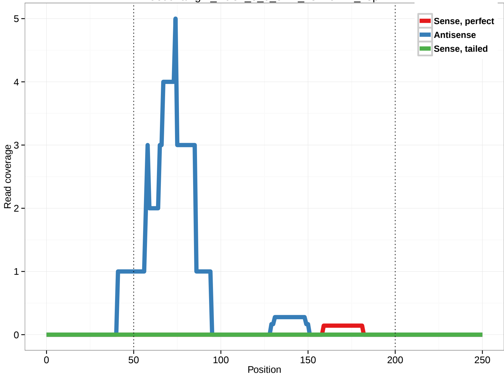
uc001awg.2_intron_5_0_chr1_15719714_f.5p
