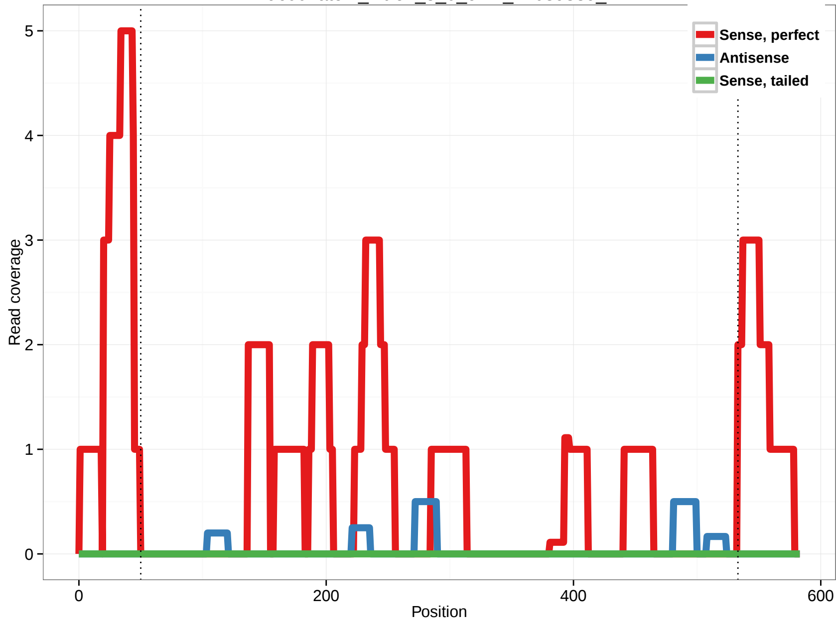
uc001ato.1_intron_5_0_chr1_12089339_f
