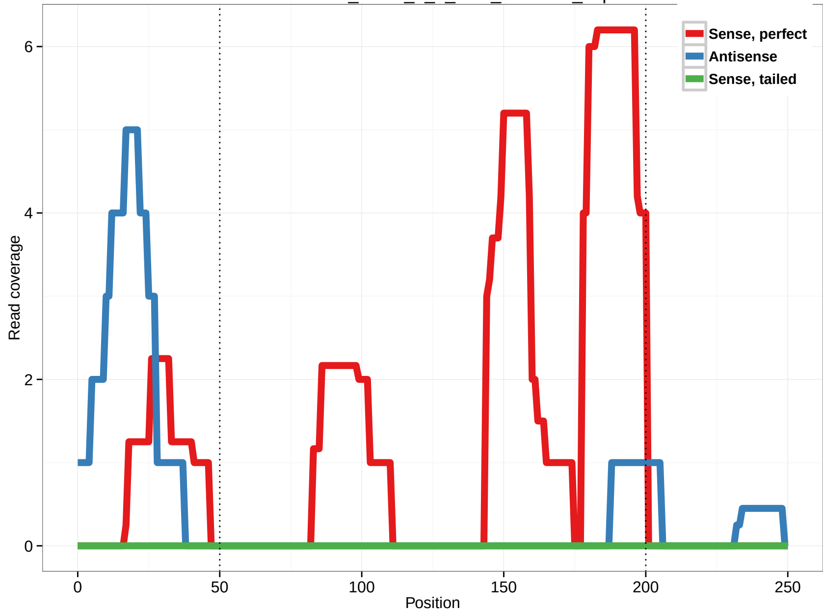
uc001aoe.1_intron_2_0_chr1_6690414_f.3p
