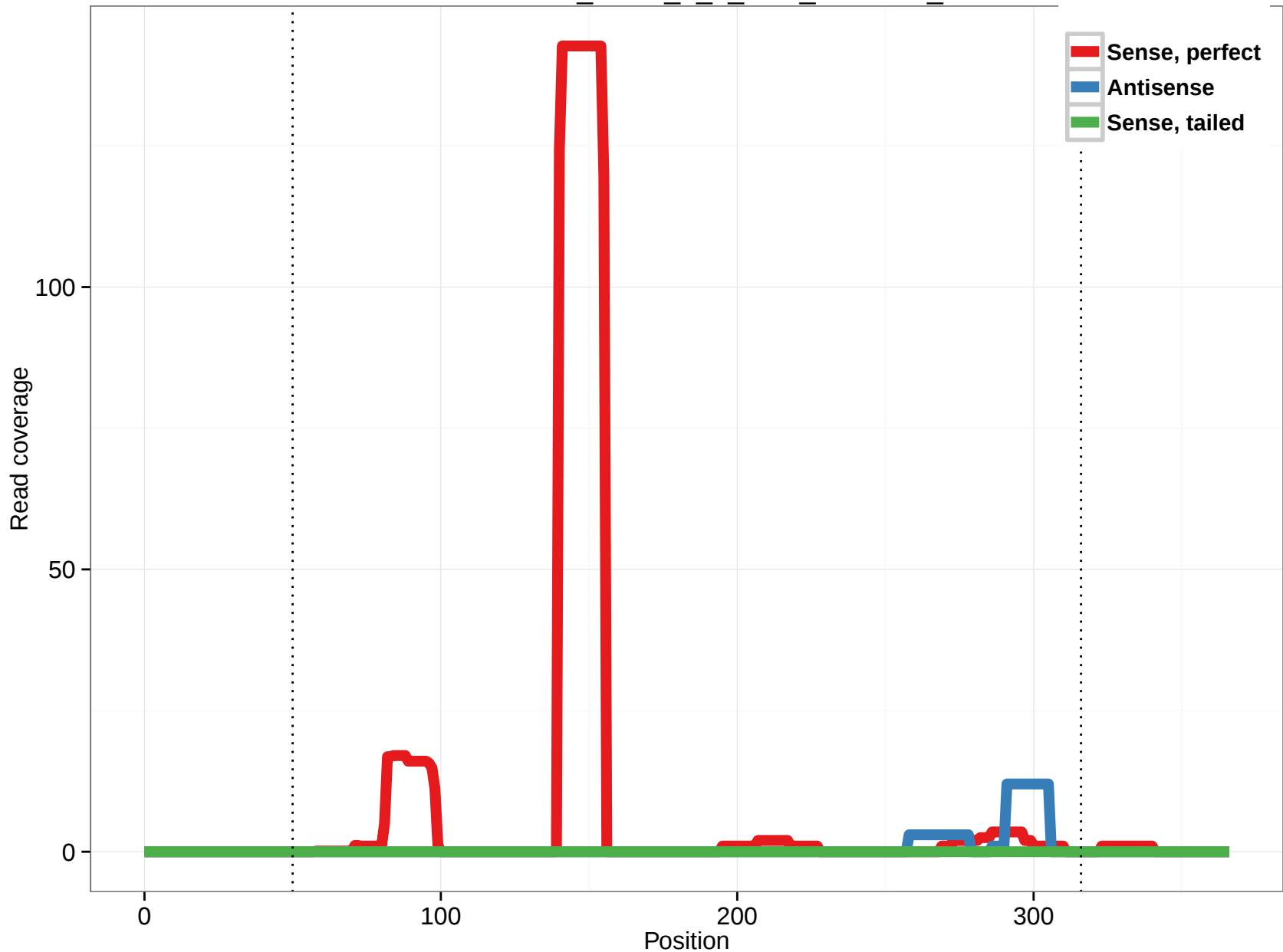
uc001amx.2_intron_1_0_chr1_6479401_r
