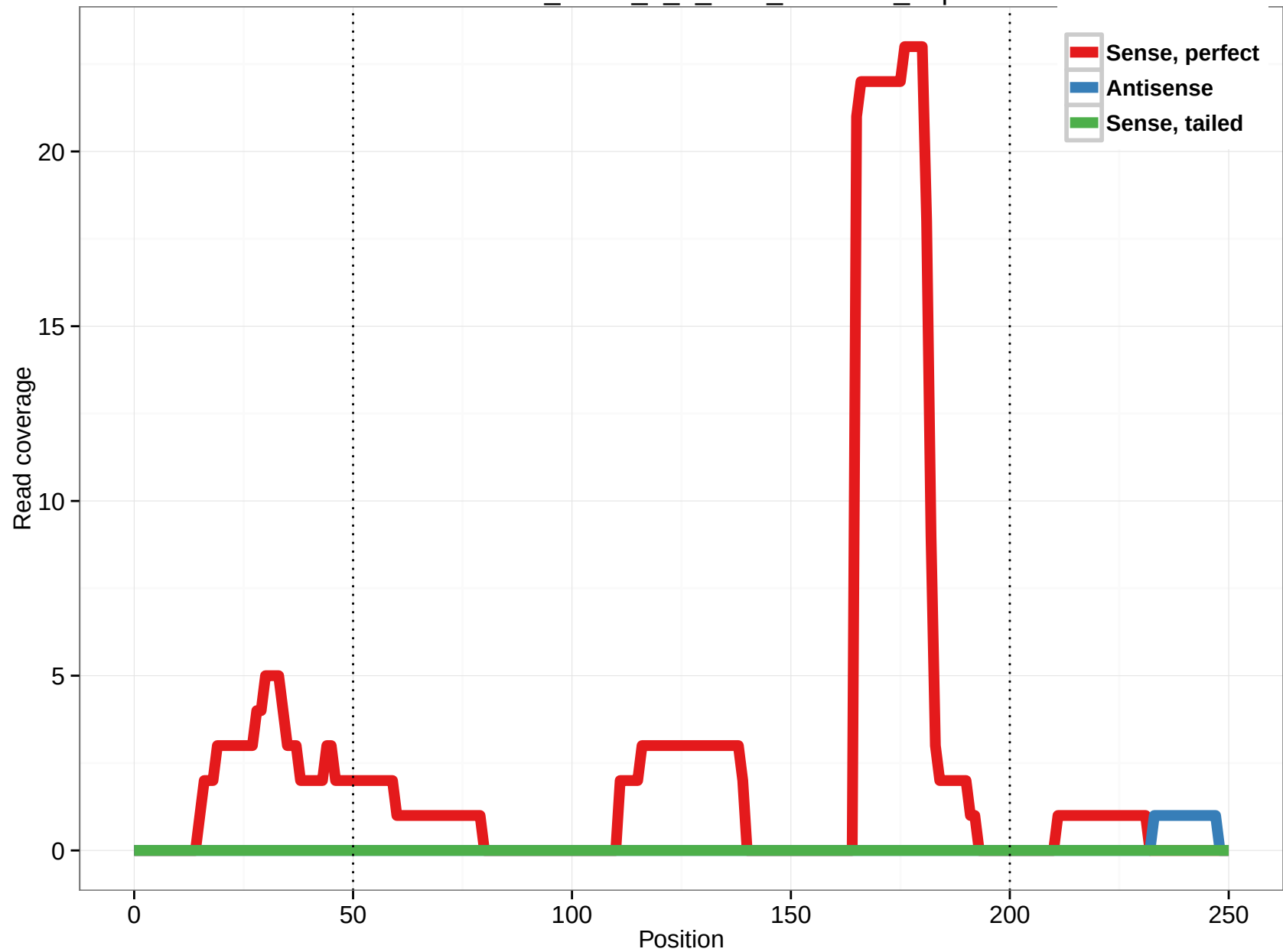
uc001aie.2_intron_8_0_chr1_1688750_r.5p
