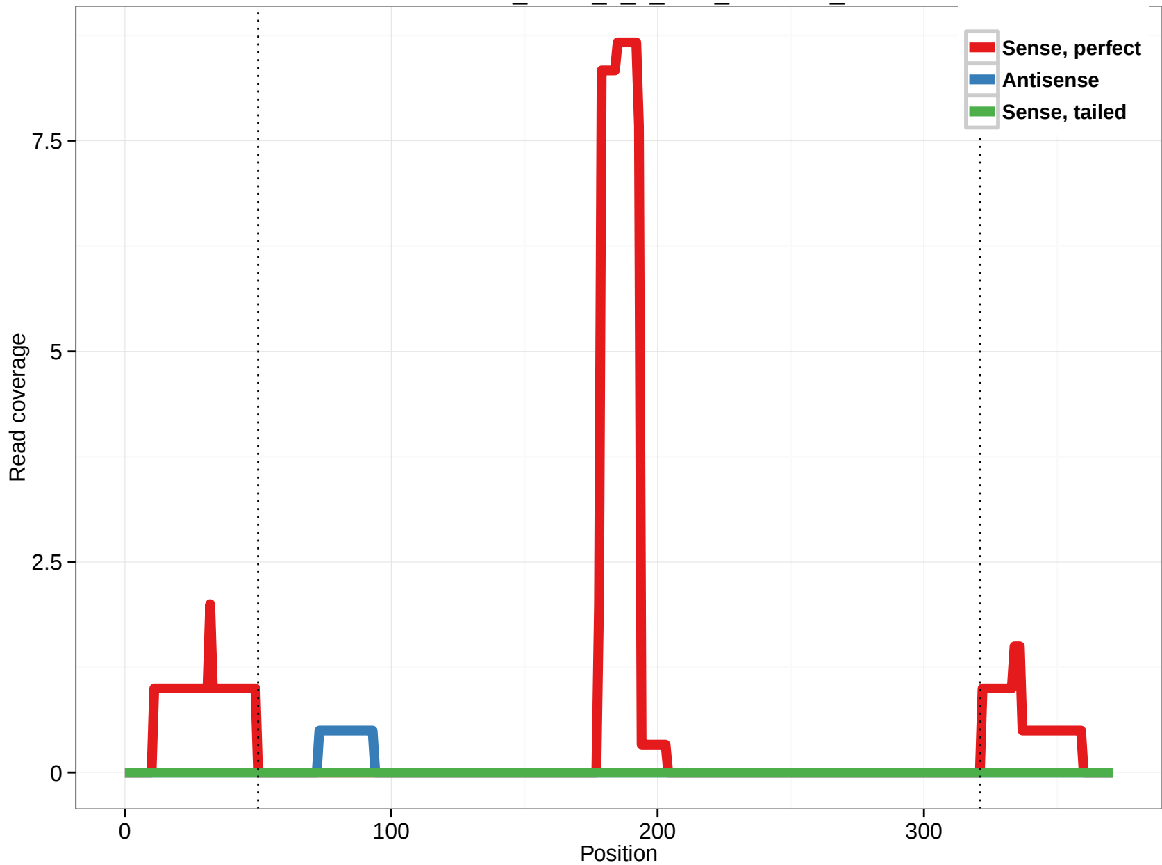
uc001afz.1_intron_8_0_chr1_1458948_f
