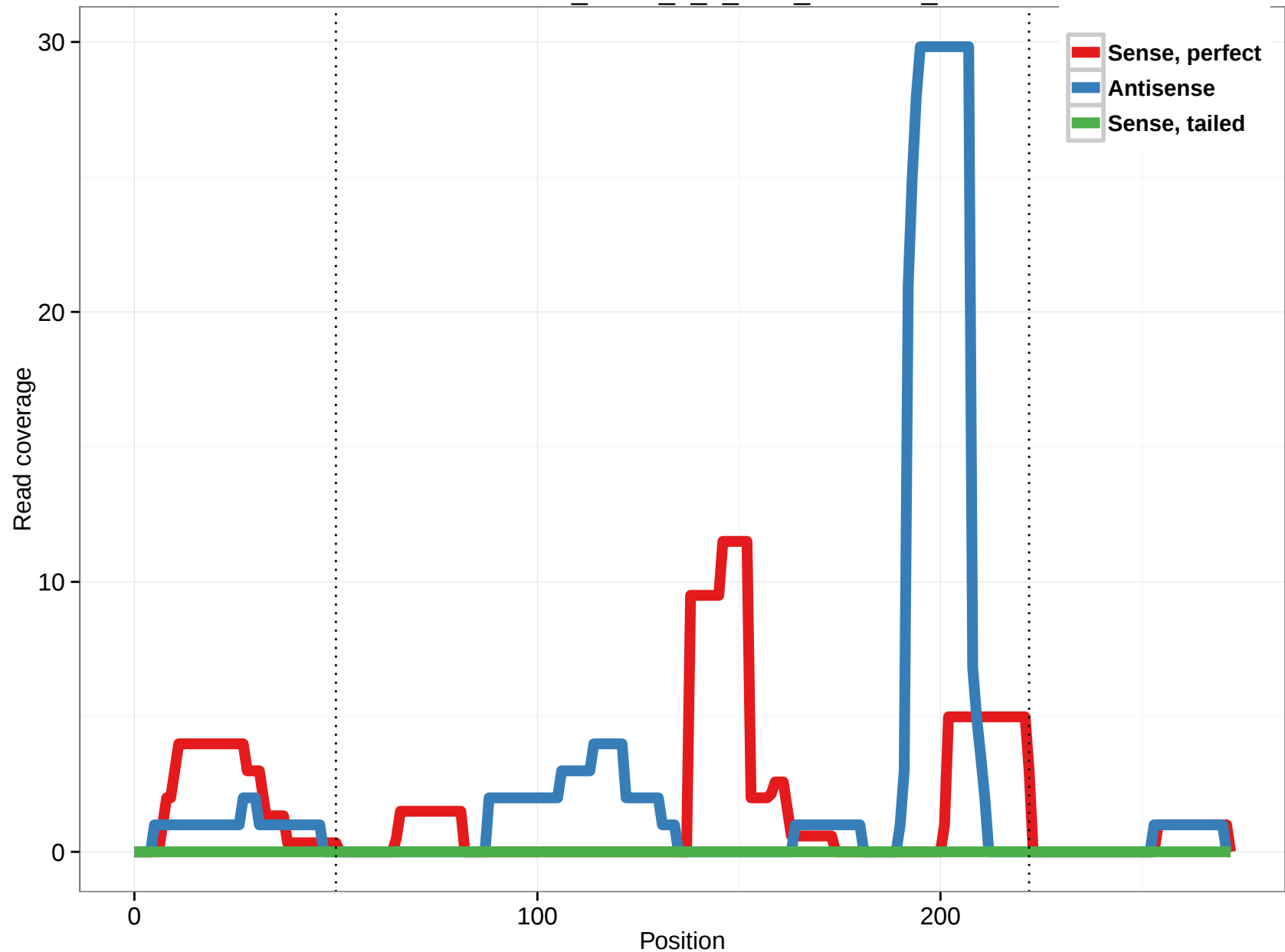
uc001aew.2_intron_4_0_chr1_1289890_r
