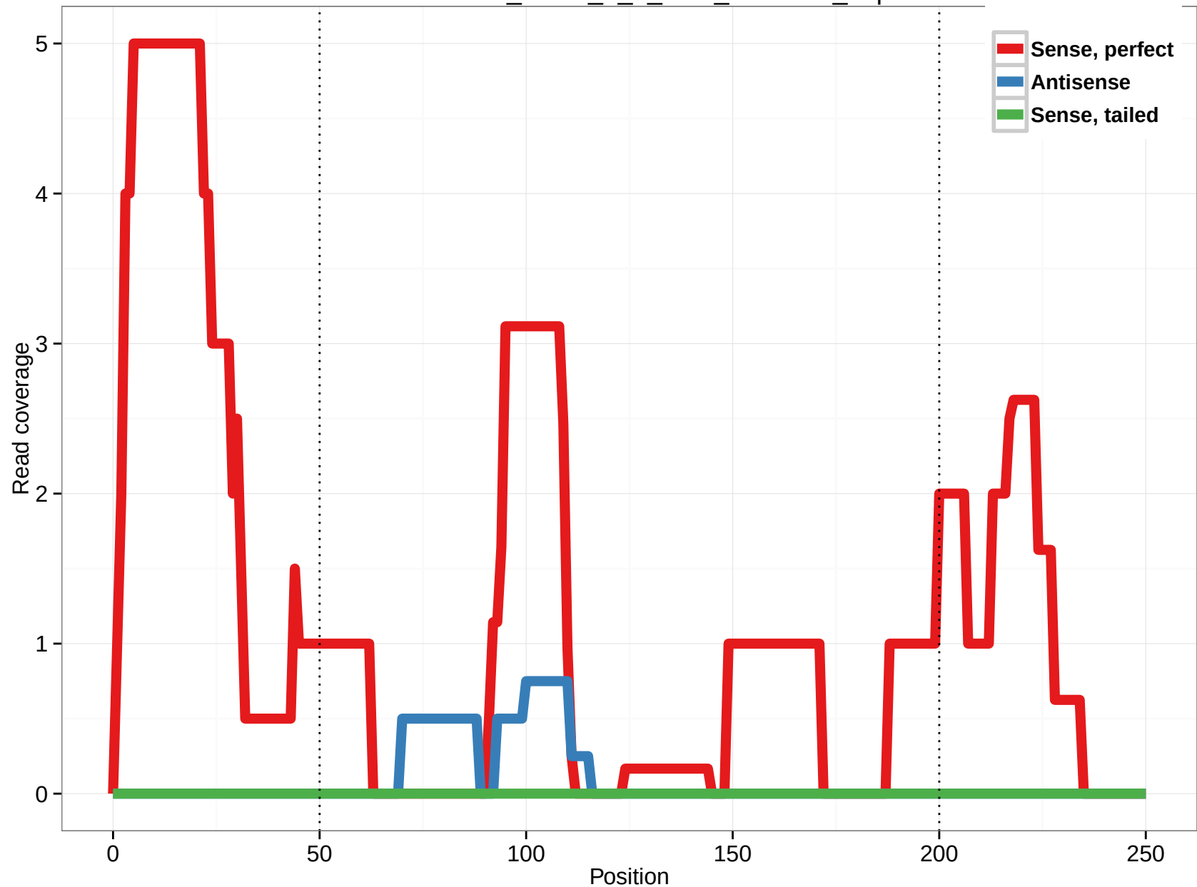
uc001adu.1_intron_4_0_chr1_1219471_f.5p
