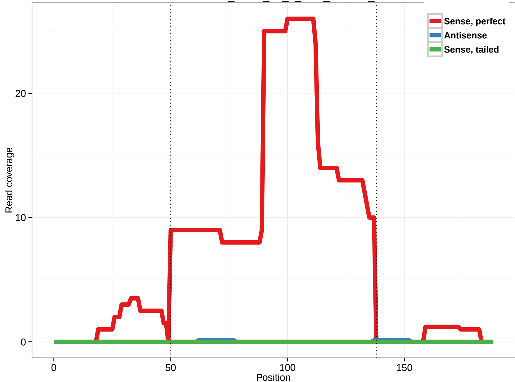
uc001ack.1_intron_20_0_chr1_983068_f
