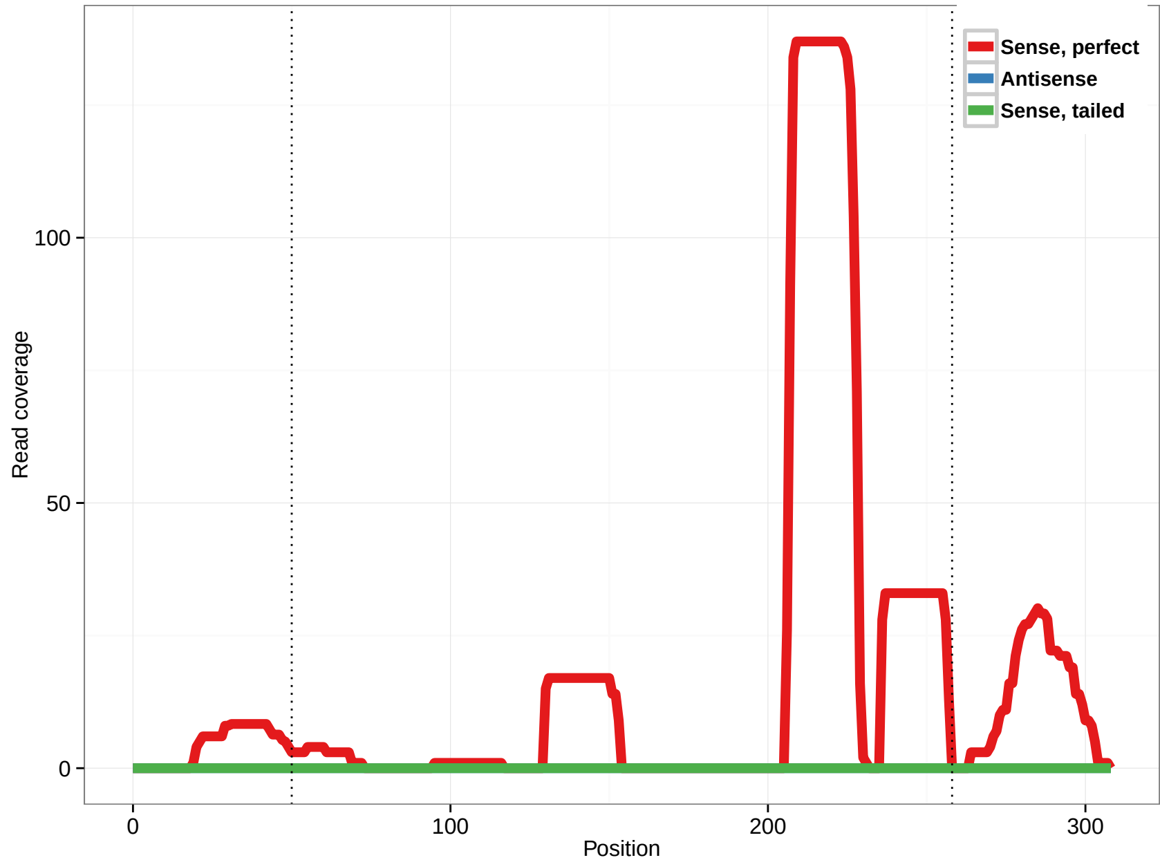
hsa-mir-6871
