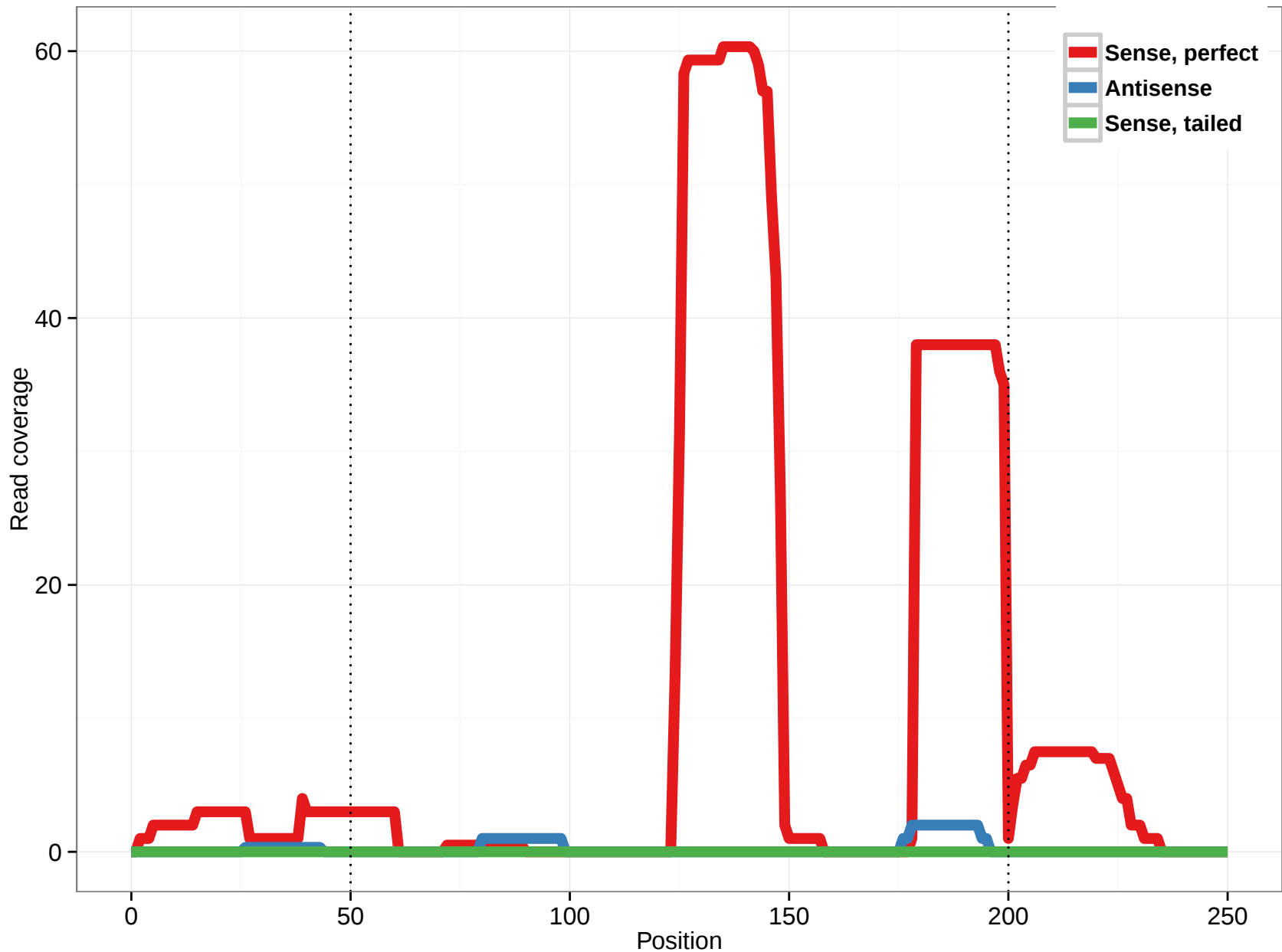
hsa-mir-6780b
