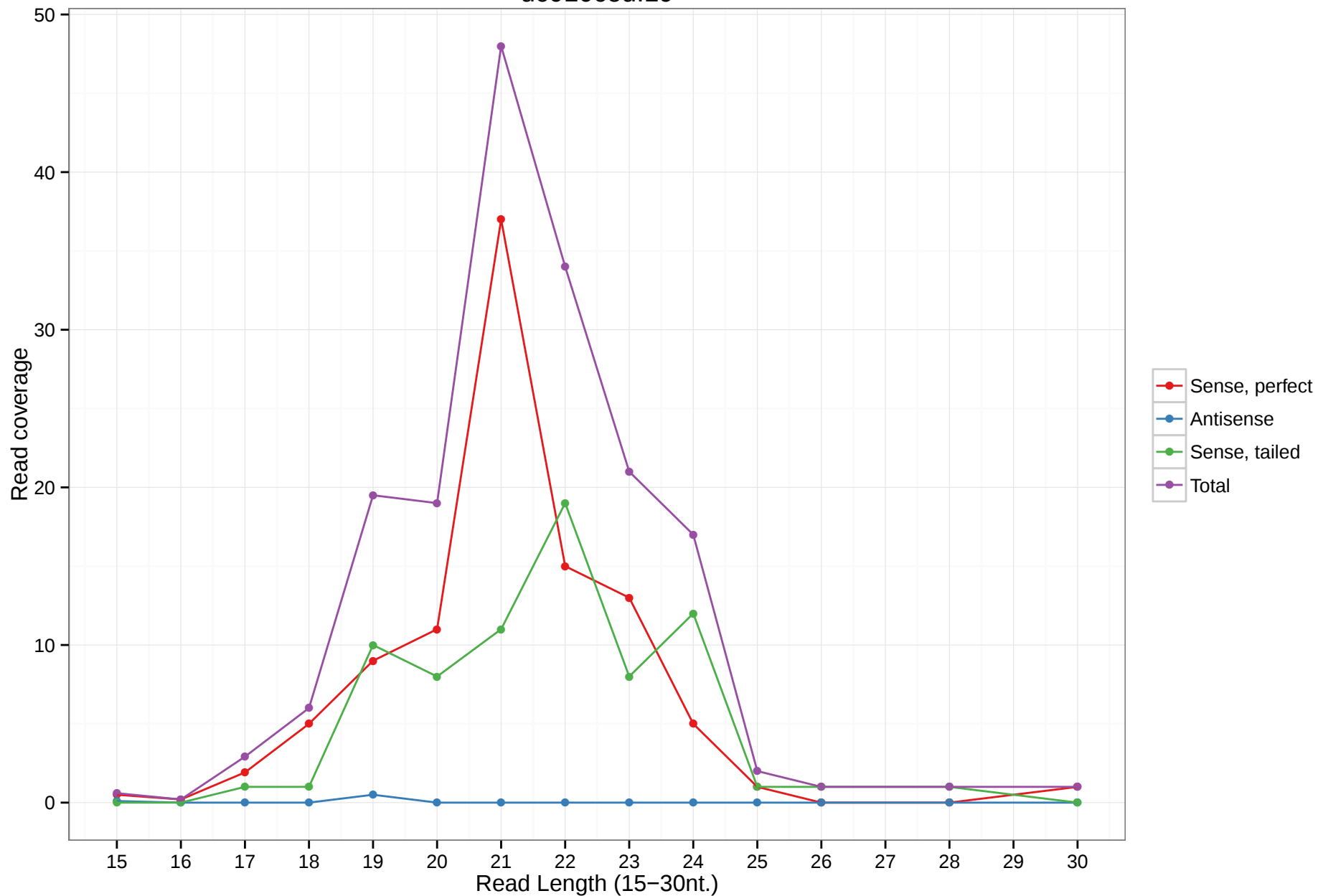
uc010ceu.19
