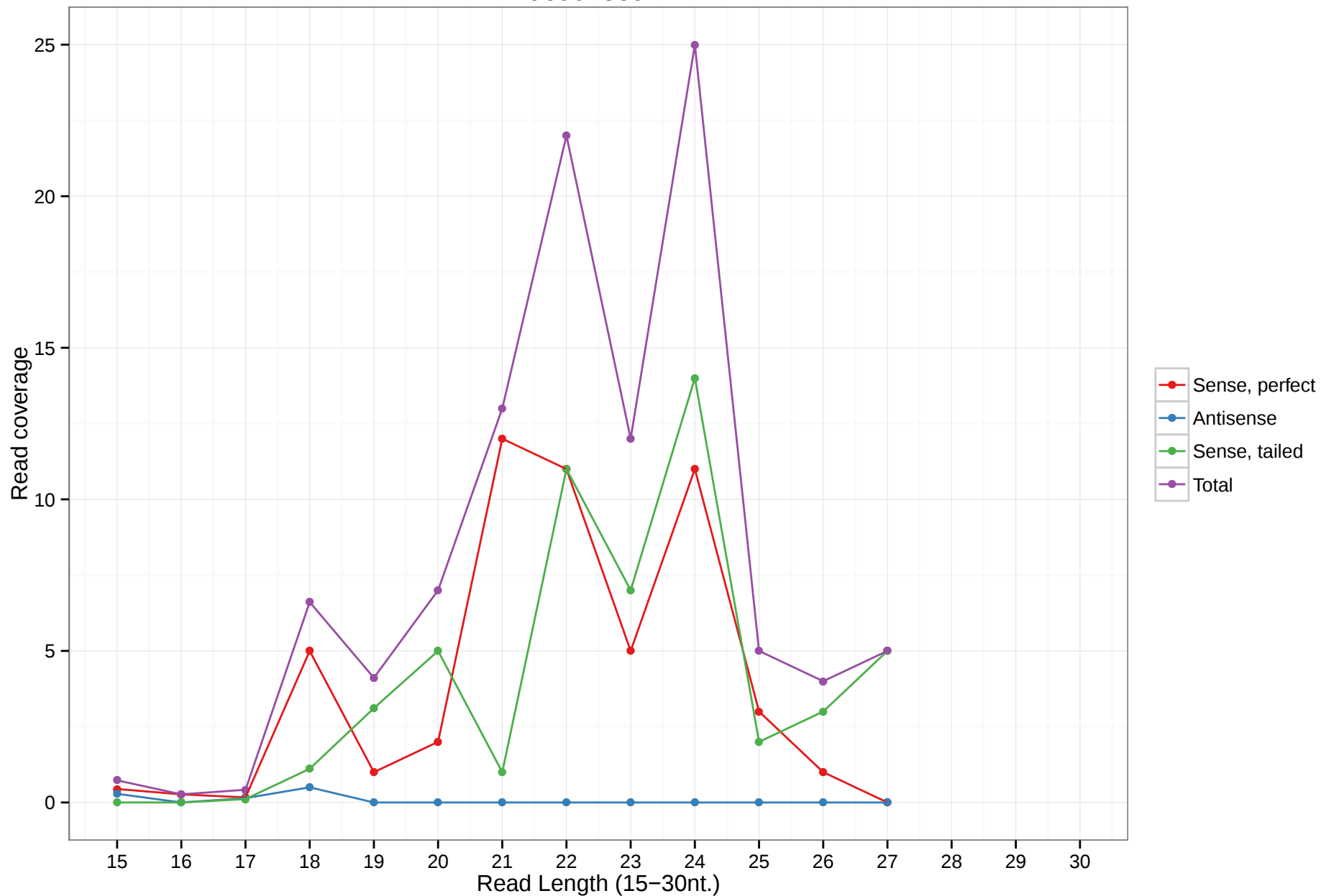
uc002oou.2
