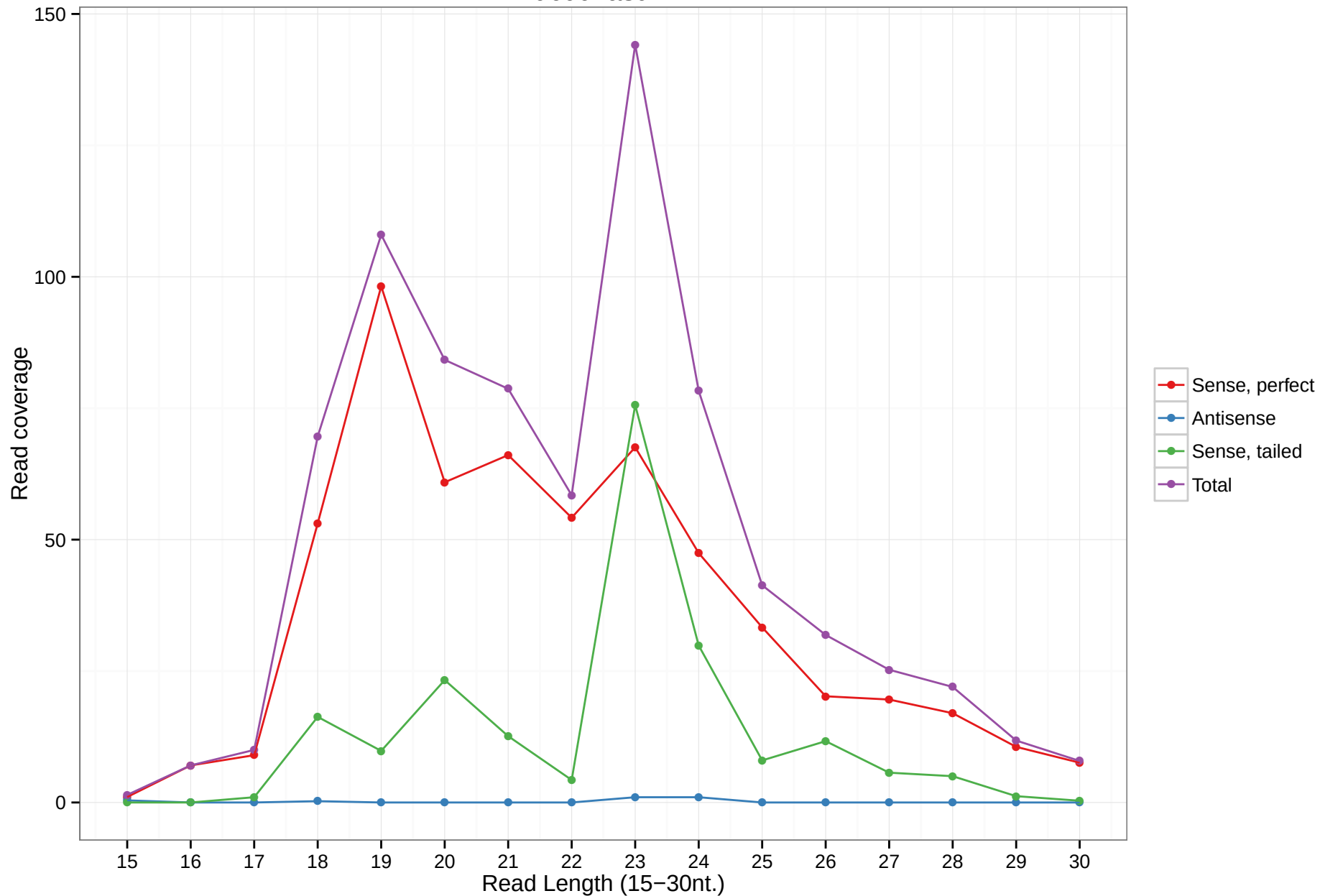
uc002asd.2
